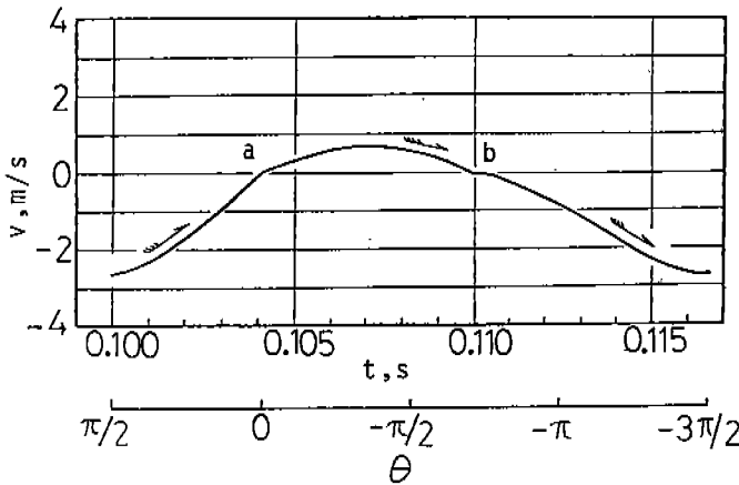
Fig. 8 Sliding velocity between vane and piston
