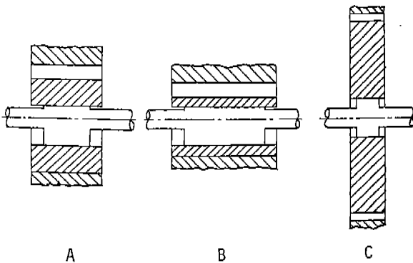
Fig. 9 Cross sections of three example cases
