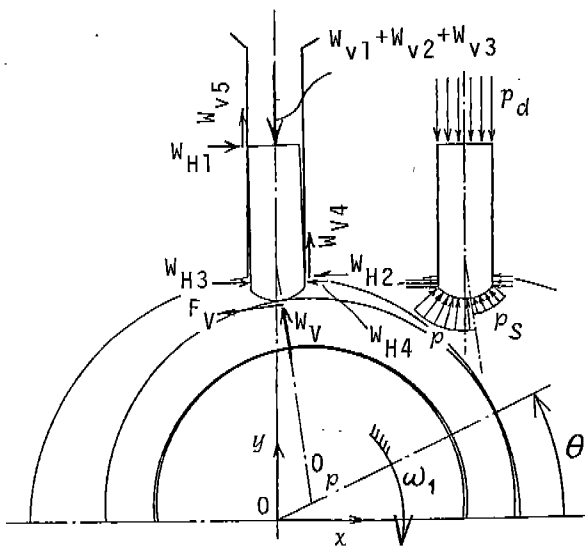
Fig. 3 Forces acting on vane
