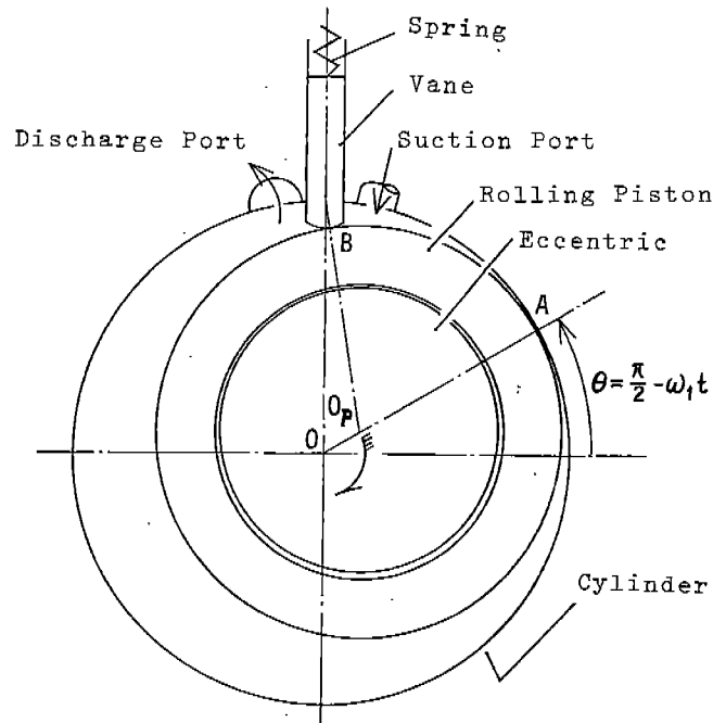
Fig. 1 Cross-section of a typical rolling piston compressor
