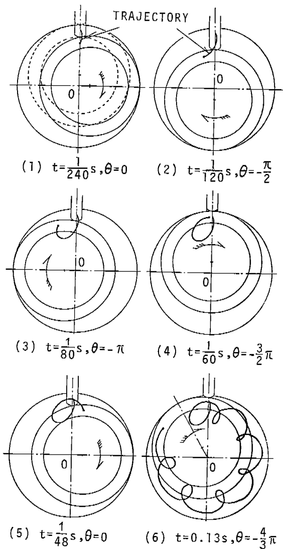
Fig. 5 Trajectory of a point on side surface of rolling piston
