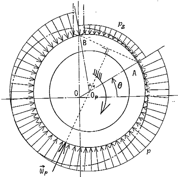
Fig. 2 Pressure distribution on rolling piston
