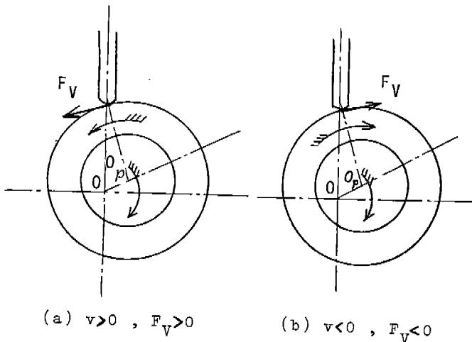
Fig. 4 Two kinds of relative motions between vane and rolling piston
