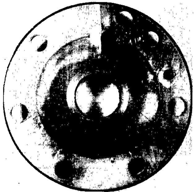
Fig. 6 Abrasive tracks on cylinder head
