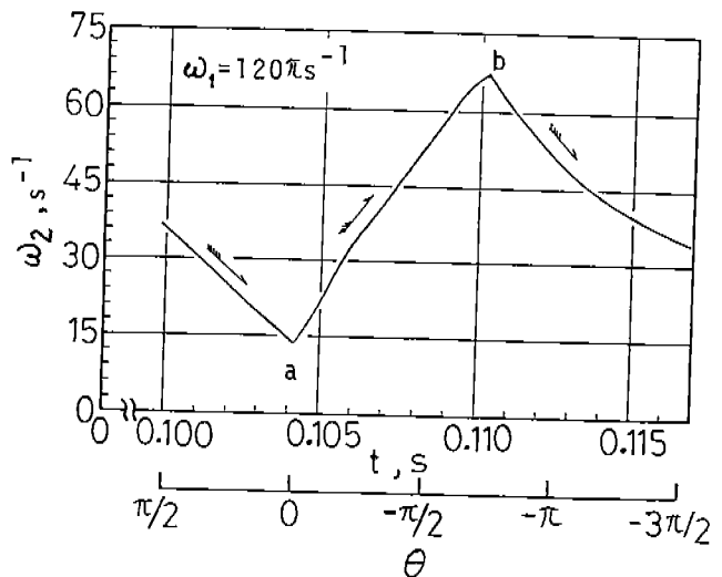
Fig. 7 Angular velocity of rolling piston
