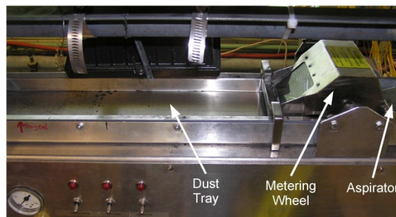
Figure 4 Dust Injector
