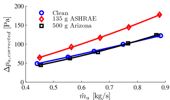
Figure 7 Pressure drop of HXB with fouling
