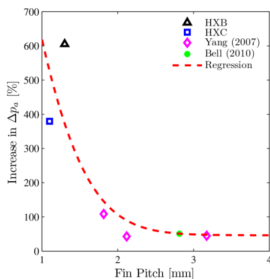
Figure 13: Increase in air-side pressure drop as a function of fin pitch for louvered fins with 1612.5 g/m 2 ASHRAE dust injected
