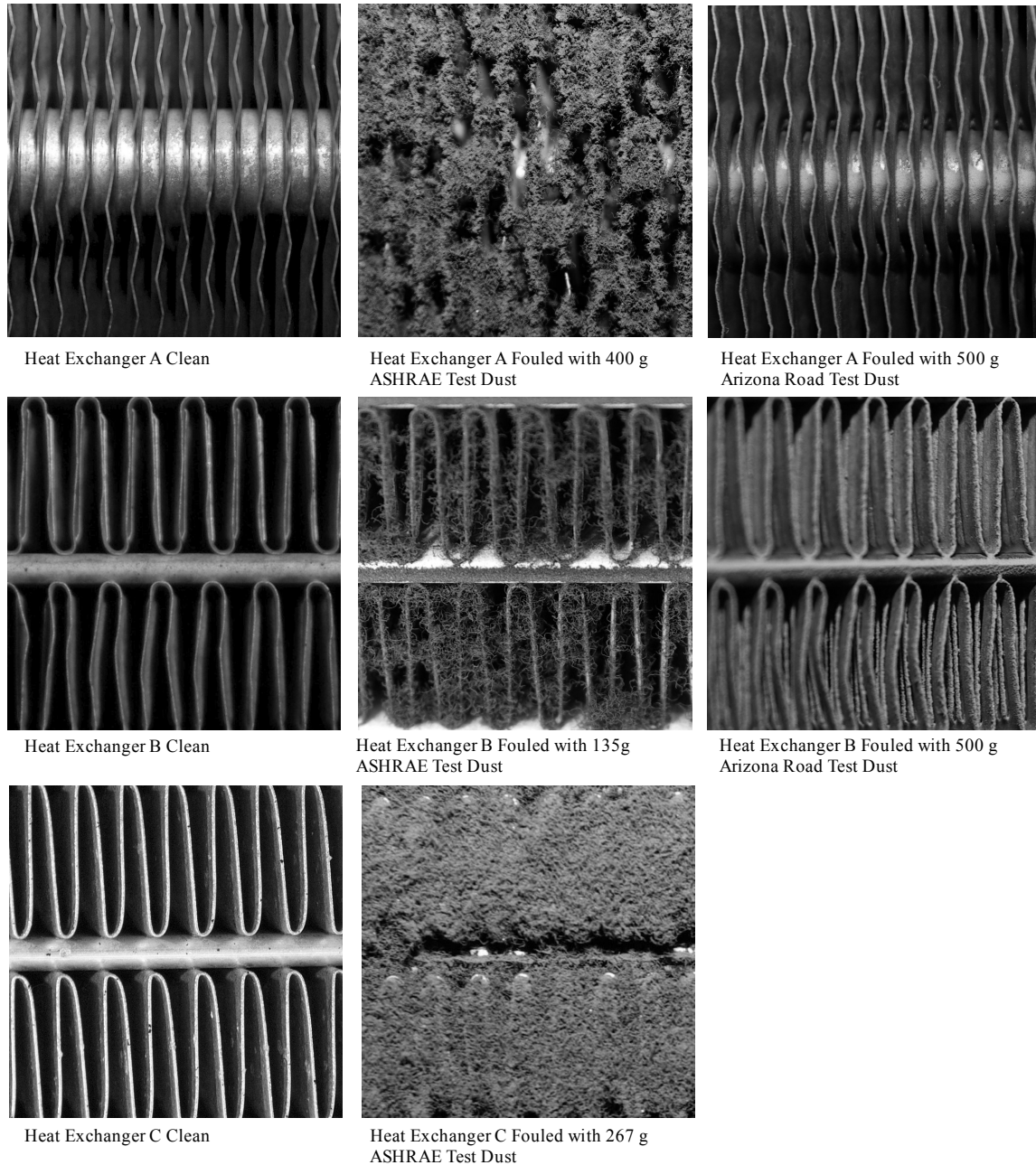
Figure 9 Macro photographs of heat exchangers fouled with dust
