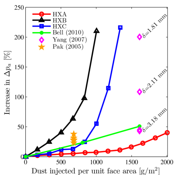
Figure 12: Literature survey of impact of ASHRAE Dust Fouling ( \delta : Fin Pitch)
