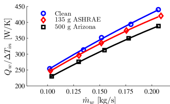
Figure 8 Heat transfer of HXB with fouling
