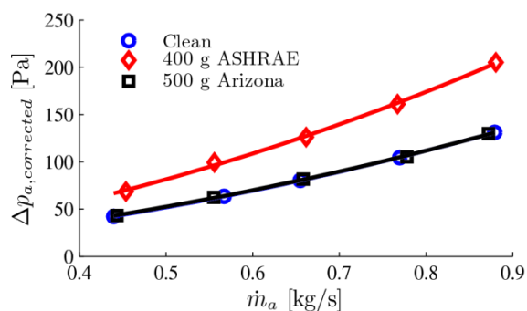
Figure 5 Pressure drop of HXA with fouling
