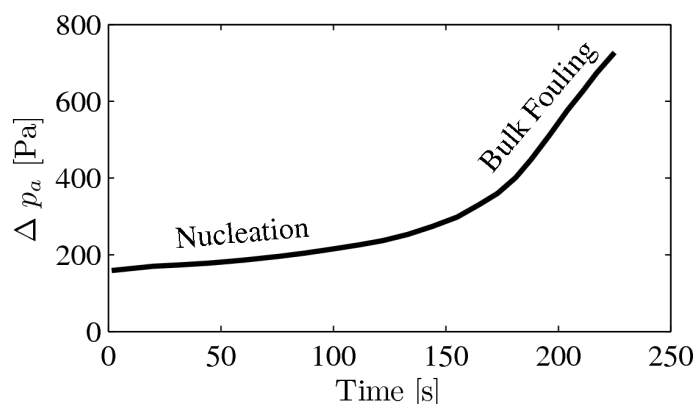
Figure 10 Evolution of the air-side pressure drop during the fouling process (Adapted from Mason et al. (2006))
