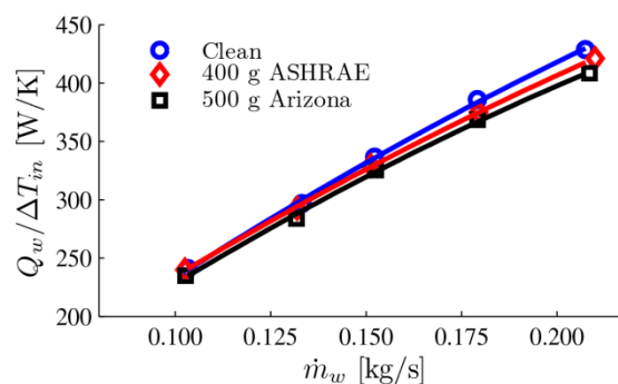
Figure 6 Heat transfer of HXA with fouling
