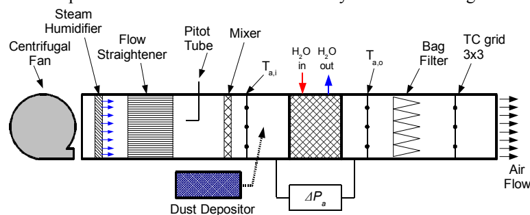
Figure 1 Schematic of Wind Tunnel used for heat exchanger testing
