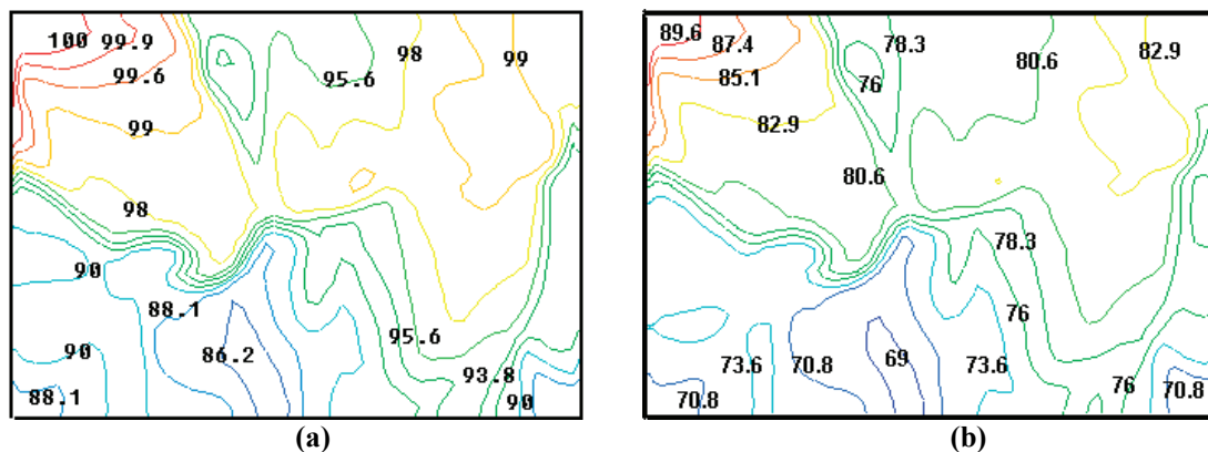
Fig.6 Relative humidity distributions on the ceiling panels: (a) Conventional system; (b) Desiccant system
