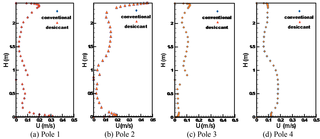
Fig.11 Vertical profiles of air velocity in several representative locations of the room.
