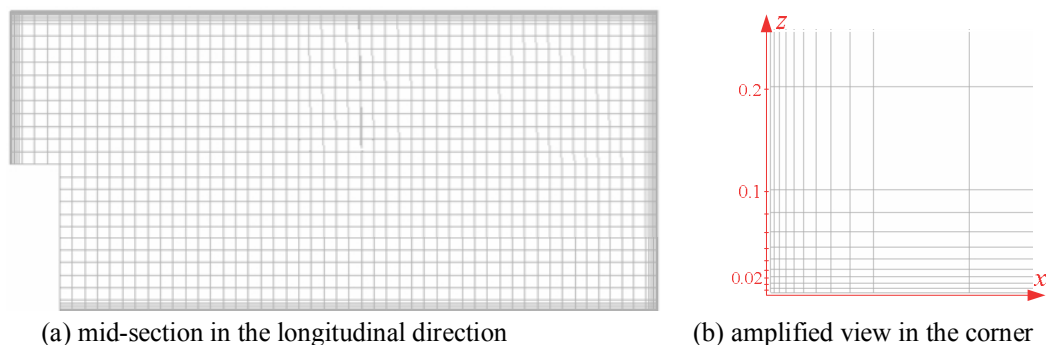
Fig.3 Grid distribution used for the conference room
