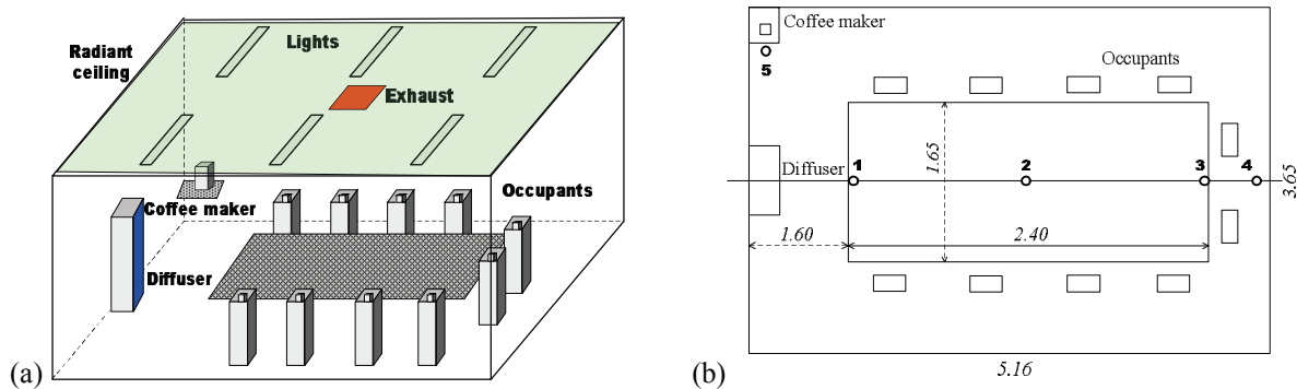
Fig.2 Conference room model for analysis: (a) conference room layout; (b) plan view of the conference room.
