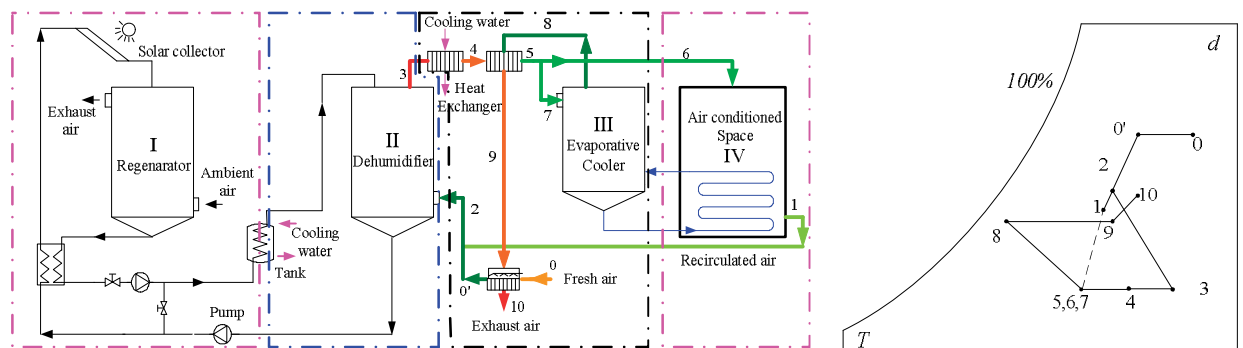
(a) System sketch (b) Air conditioning processes in psychrometric chart Fig.1 A new liquid desiccant dehumidification/radiant cooling system
