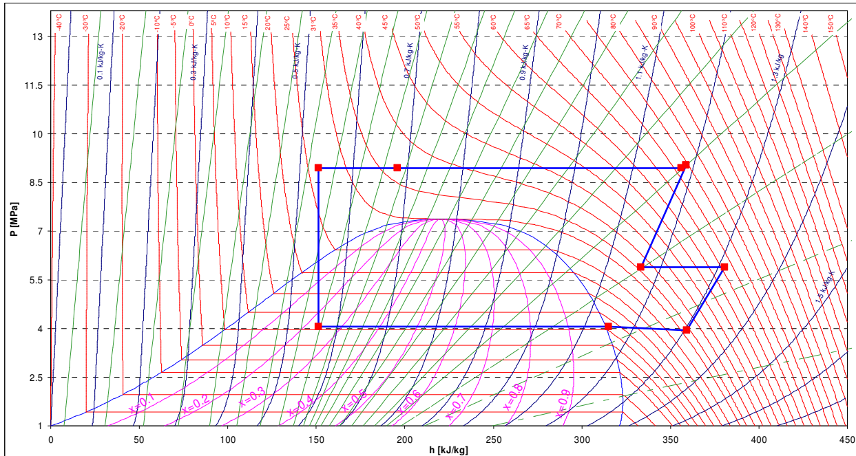
Figure 1. Pressure-enthalpy diagram of employed cycle
