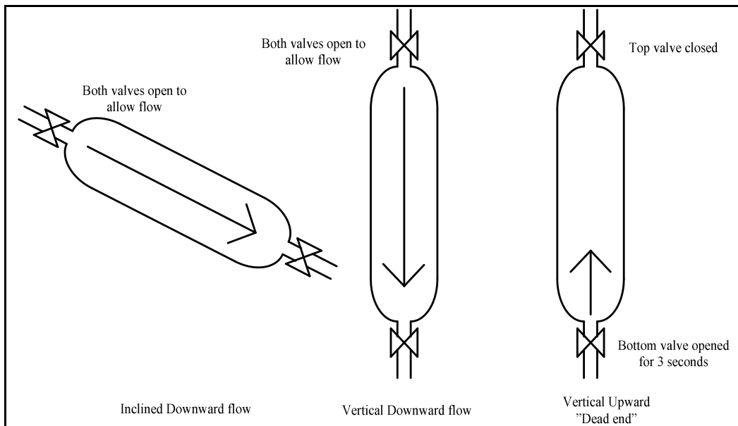
Figure 6. Orientations of the sample cylinder with valves
