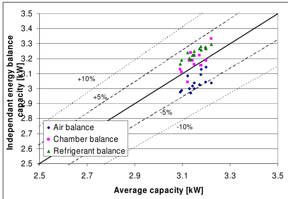
Figure 4. Evaporator energy balances
