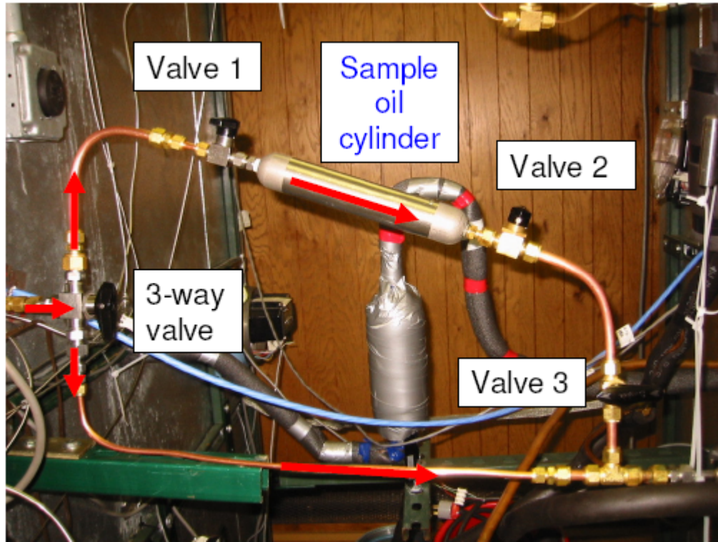
Figure 5. Inclined downward sample cylinder orientation, with valves (O'Connor)
