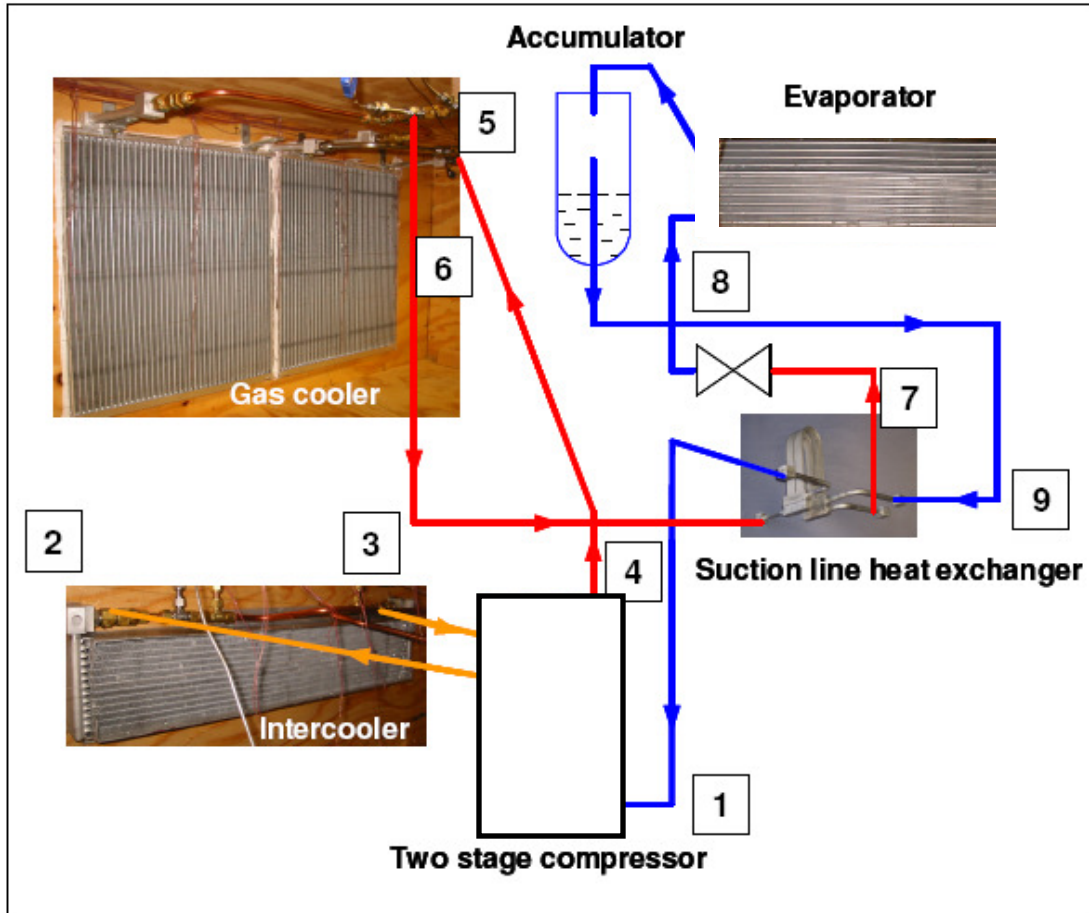
Figure 2. Components with schematic of pipe routing (O'Connor)
