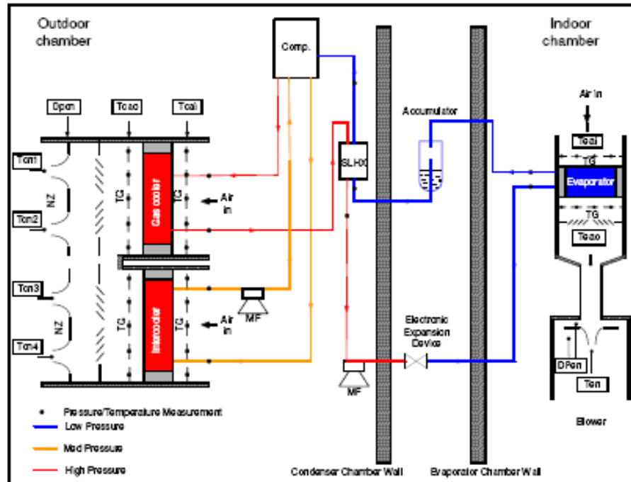
Figure 3. Diagram of experiment setup
