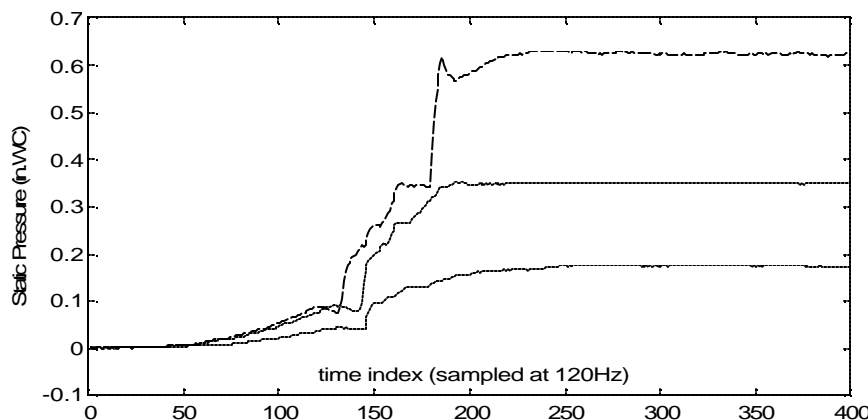
Figure 7. Condenser fan pressure start transients, mean of repetitions for each fault level: 0% blockage (solid), 14% blockage (dotted), and 39% blockage (dashed).
