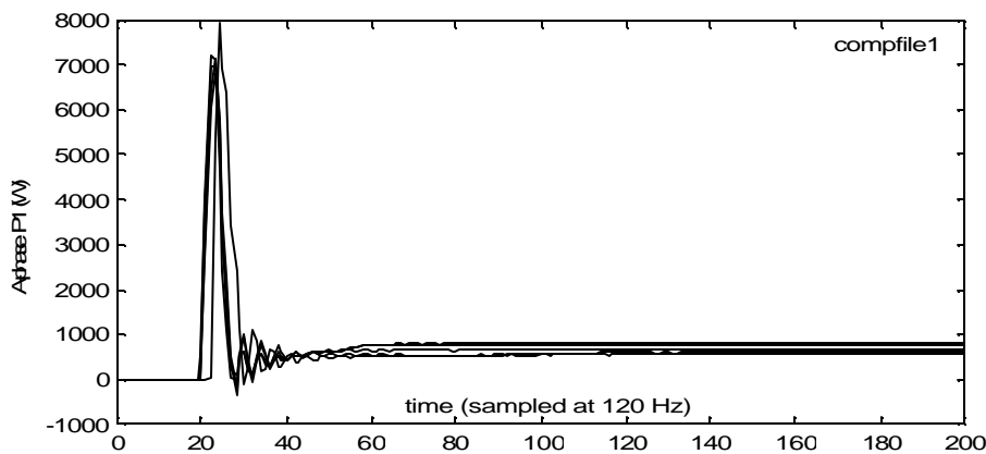
Figure 1. Five compressor starts with no pressure relief.
