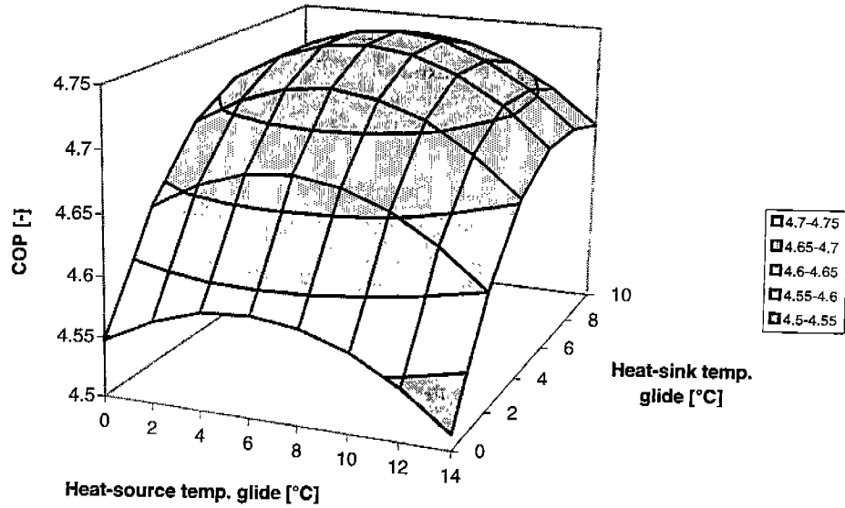
Figure 6. COP versus heat-sink and heat-source temperature glides (DT version of CYCLE-11, cooling, T_{\text{outdoor}}=35 °C, T_{\text{indoor}}=26.7 °C, cross-flow condenser, counter-flow evaporator)
