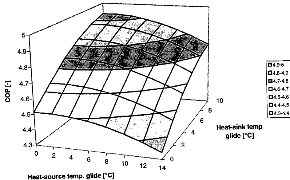
Figure 5. COP versus heat-sink and heat-source glides (DT version of CYCLE-11, cooling, T_{\text{outdoor}}=35\text{ }^{\circ}\text{C} , T_{\text{indoor}}=26.7\text{ }^{\circ}\text{C} , cross-flow evaporator, counter-flow condenser)
