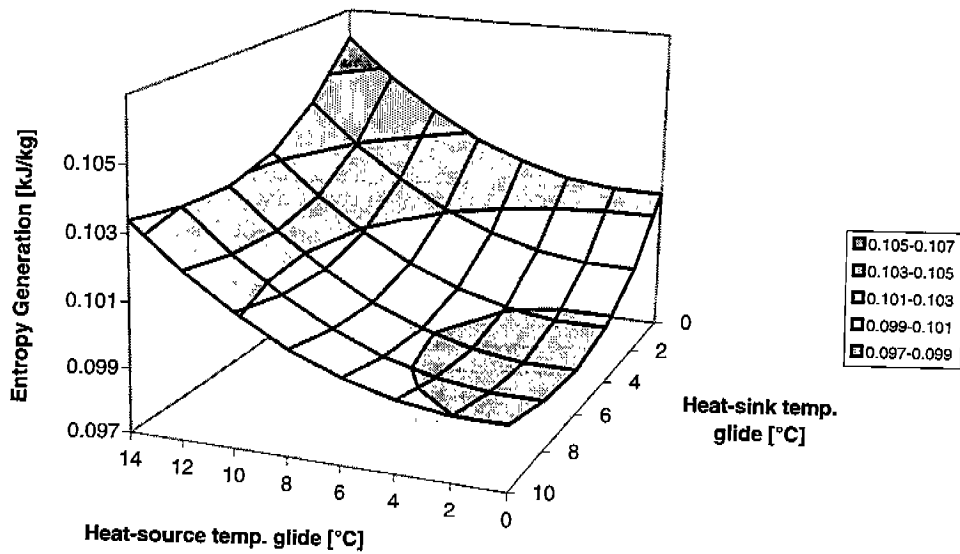
Figure 7. Entropy generation versus heat-sink and heat-source temperature glides (DT version of CYCLE-11, cooling, T_{\text{outdoor}}=35 °C, T_{\text{indoor}}=26.7 °C, cross-flow evaporator and cross-flow condenser)
