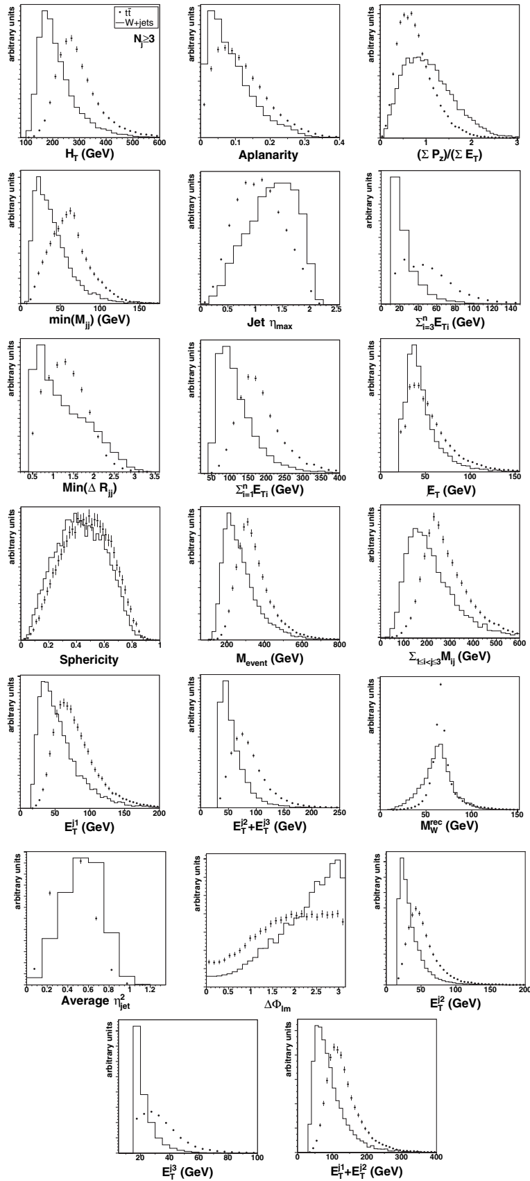
FIG. 3. Shape comparison of PYTHIA t\bar{t} to ALPGEN + HERWIG W + 3p Monte Carlo simulation for the 20 kinematic and topological properties considered for the W + \geq 3 jets sample. The distributions are normalized to equal area.
