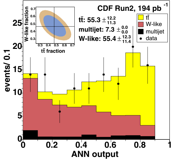
FIG. 18 (color online). Distribution of observed ANN output in the W + \geq 4 jets sample, compared with the result of the fit. The inset shows the 1- and 2-standard deviation contours of the free parameters in the fit, normalized to the total number of observed events. The contribution of multijet background to the fit is fixed.
