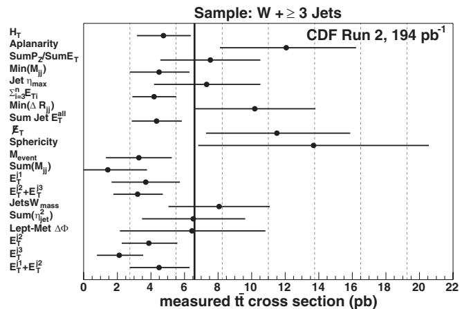
FIG. 19. Measured t\bar{t} cross section in the W + \geq 3 jets sample for all 20 kinematic and topological properties considered. The uncertainty is statistical only, the vertical line shows the measured cross section with the ANN of 6.6 pb.
