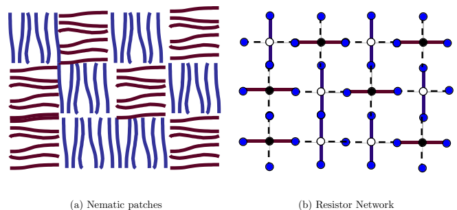
FIG. 1 (color online). Mapping of nematic patches to random resistor networks. (a) Configurations of nematic patches generated by the random field Ising model. (b) Corresponding resistor network, modeling local anisotropic conduction in each nematic patch. Solid lines are small resistors, and dotted lines are large ones.
