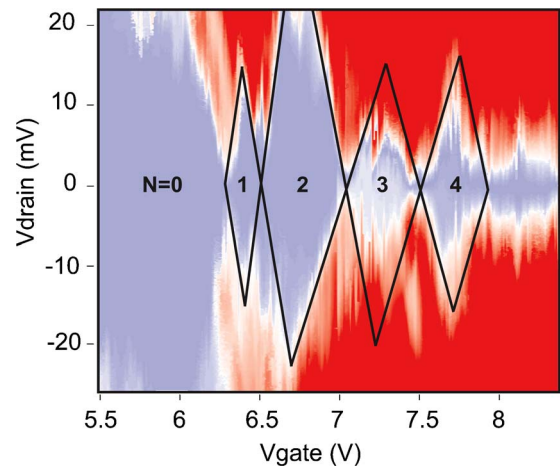
FIG. 3. (Color online) Diamond chart of an enhancement-mode SET measured at 4.2 K.
