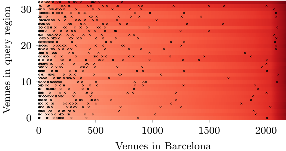
Figure 4: Intuition behind our pruning strategy: for two neighborhoods with small EMD, the venues of one neighborhood are in the k -NN set of the venues of the other.
