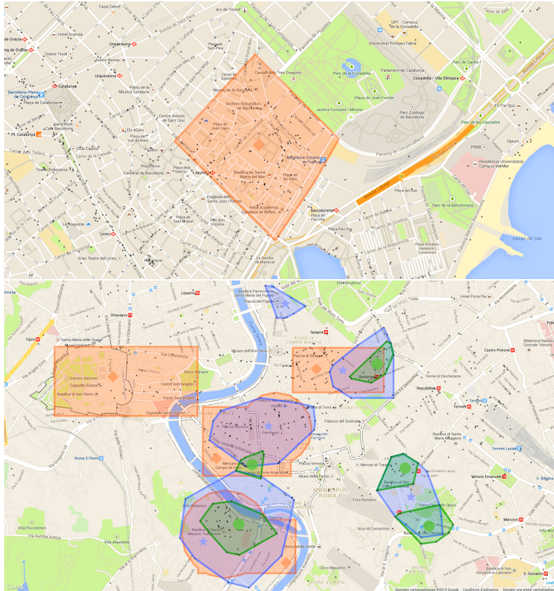
Figure 7: Top: the neighborhood query in Barcelona ( La Ribera ). Bottom: the results in Rome match the ground truth (in orange), both from Barcelona (green) and Paris (blue, the query is showed in blue in Figure 3).
