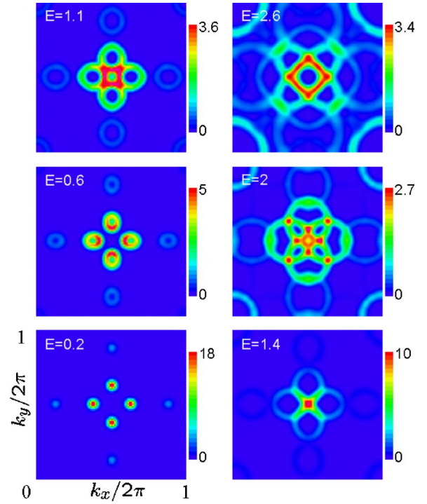
FIG. 5. (Color online) VB4 at J_b=-0.4J_a : Constant energy cuts with windows 0.2J_a for twinned vertical, bond-centered stripes of spacing d=4 at J_b=-0.4J_a . The energy E is in units of J_aS .
