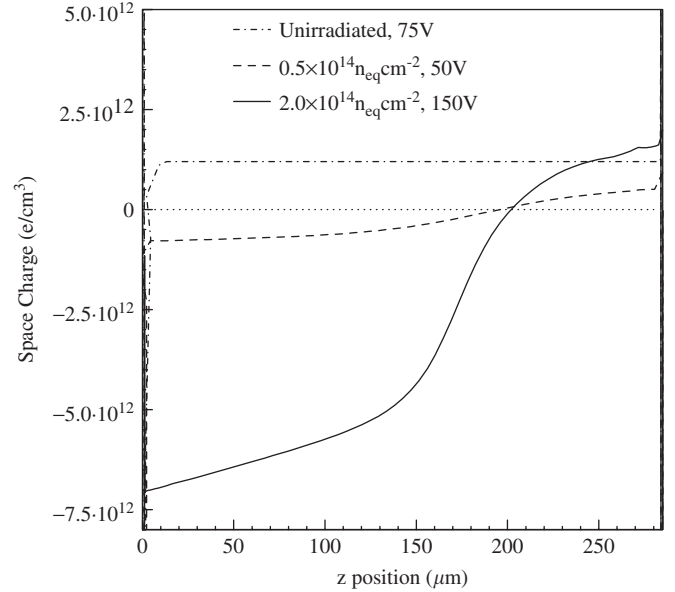
Fig. 8. The simulated space charge density at T = -10^\circ\text{C} as a function of the z coordinate for fluences of \Phi = 0.5 \times 10^{14} \text{ n}_{\text{eq}}/\text{cm}^2 and \Phi = 2 \times 10^{14} \text{ n}_{\text{eq}}/\text{cm}^2 .
