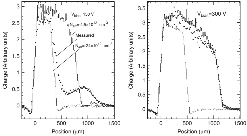
Fig. 3. The measured and simulated charge collection profiles for a sensor at T = -10^\circ\text{C} irradiated to a fluence of \Phi = 5.9 \times 10^{14} \text{ n}_{\text{eq}}/\text{cm}^2 . The profiles measured at bias voltages of 150 and 300 V are shown as solid dots. The full histograms are the simulated profiles for a constant effective doping N_{\text{eff}} = 4.5 \times 10^{12} \text{ cm}^{-3} of acceptor impurities. The dashed histograms are the simulated profiles for a constant effective doping N_{\text{eff}} = 24 \times 10^{12} \text{ cm}^{-3} .
