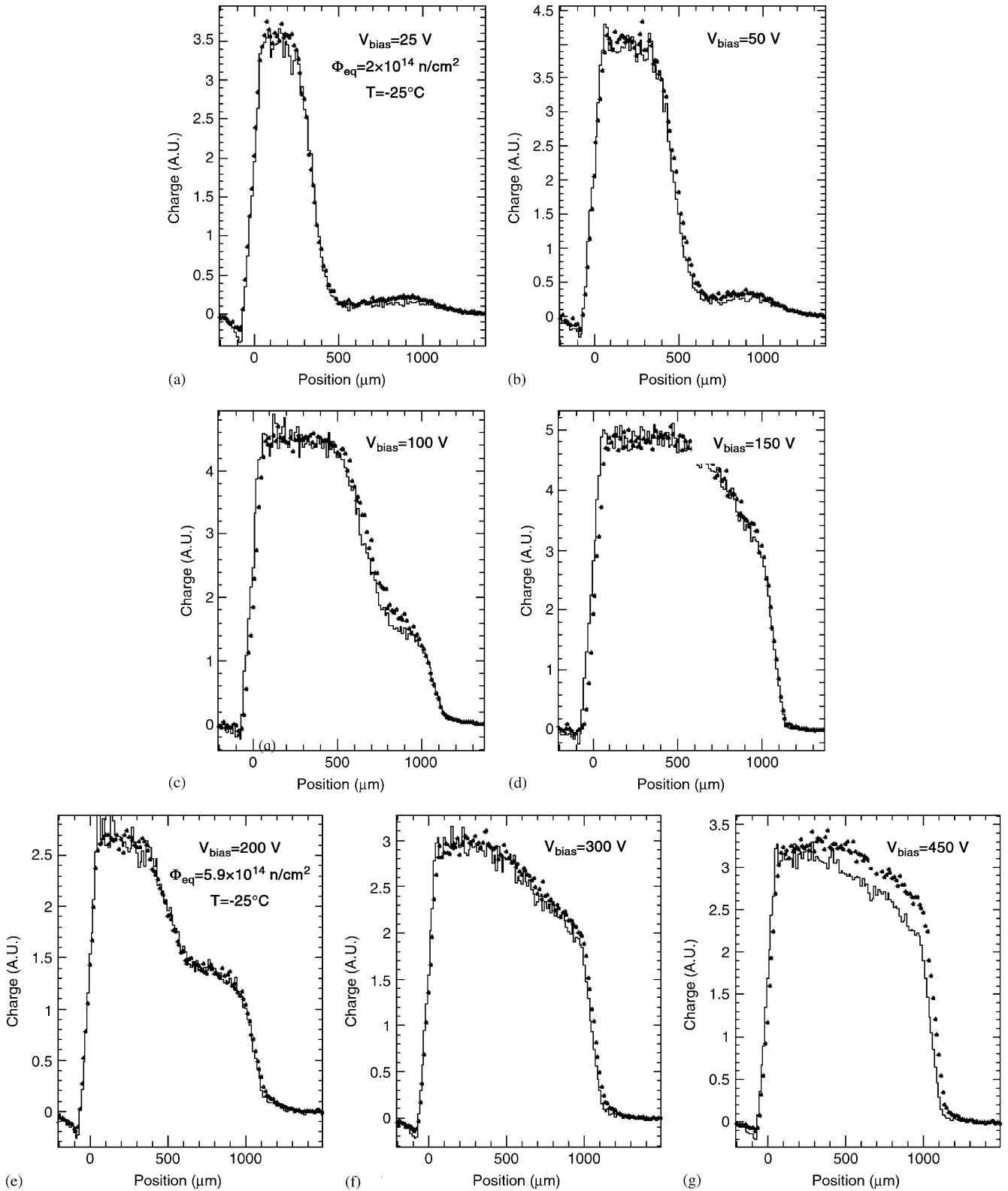
Fig. 9. Measured (full dots) and simulated (histogram) charge collection profiles at T = -25^\circ\text{C} and several bias voltages for sensors irradiated to fluences of \Phi = 2.0 \times 10^{14}\text{ n}_{\text{eq}}/\text{cm}^2 (a–d) and of \Phi = 5.9 \times 10^{14}\text{ n}_{\text{eq}}/\text{cm}^2 (e–g).
