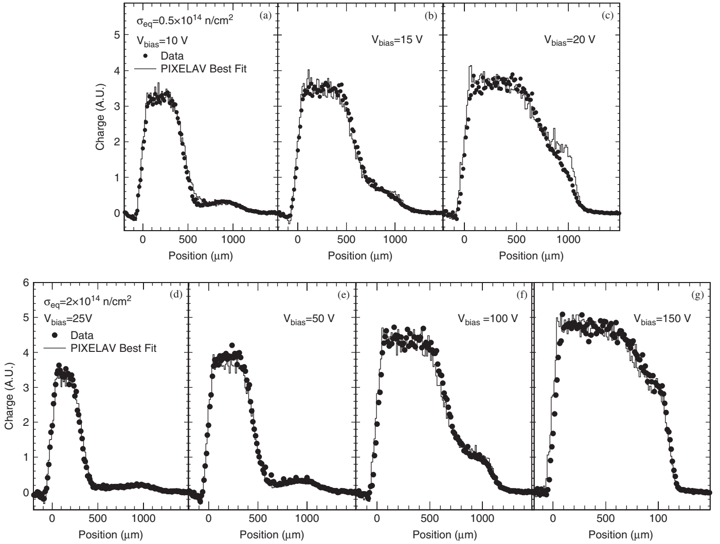
Fig. 6. Measured (full dots) and simulated (histogram) charge collection profiles for sensors irradiated to fluences of \Phi = 0.5 \times 10^{14} \text{ n}_{\text{eq}}/\text{cm}^2 (a–c) and of \Phi = 2 \times 10^{14} \text{ n}_{\text{eq}}/\text{cm}^2 (d–g), at T = -10^\circ\text{C} and several bias voltages.
