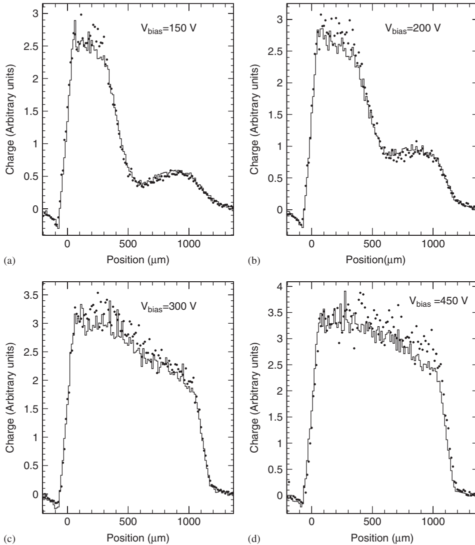
Fig. 4. The measured charge collection profiles at a temperature of -10^\circ\text{C} and bias voltages of 150, 200, 300, and 450 V are shown as solid dots for a fluence of 5.9 \times 10^{14} \text{ n}_{\text{eq}}/\text{cm}^2 . The two-trap double junction simulation is shown as the solid histogram in each plot.
