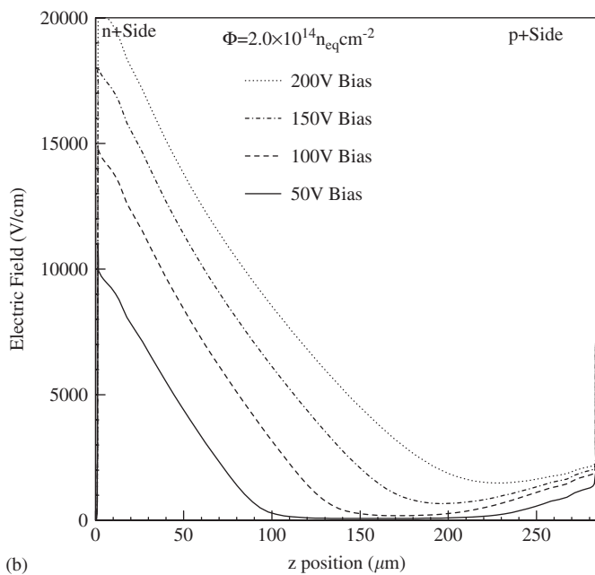
Fig. 7. The z -component of the simulated electric field at T = -10^\circ\text{C} resulting from the model best fit is shown as a function of z for a sensor irradiated to fluences of \Phi = 0.5 \times 10^{14} \text{ n}_{\text{eq}}/\text{cm}^2 (a) and \Phi = 2 \times 10^{14} \text{ n}_{\text{eq}}/\text{cm}^2 (b).
