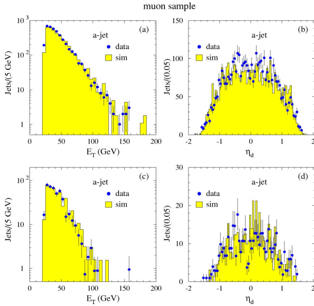
FIG. 4. Away-jet distributions in events where the muon-jet is tagged by SECVTX. (a) a -jet transverse energy; (b) a -jet pseudorapidity; (c) transverse energy of a -jets tagged by SECVTX; (d) pseudorapidity of a -jets tagged by SECVTX. Jet energies are corrected for detector effects and out-of-cone losses.
