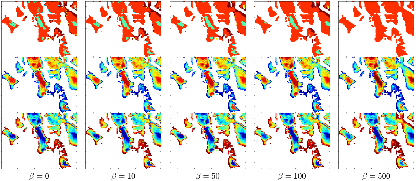
Fig. 4. Qualitative results obtained with MRF-hGLLiM-2 for orbit 61. Top row: Each pixel n is colored according to the class k maximizing p(Z_n = k | Y_n = y_n; \phi) (each class index is assigned an arbitrary color). Middle row: Proportion of CO 2 ice. Bottom row: Proportion of Dust. Concentration color codes are the same as in Fig. 2. To better appreciate the smoothing effect, a zoomed region is showed for each orbit.
