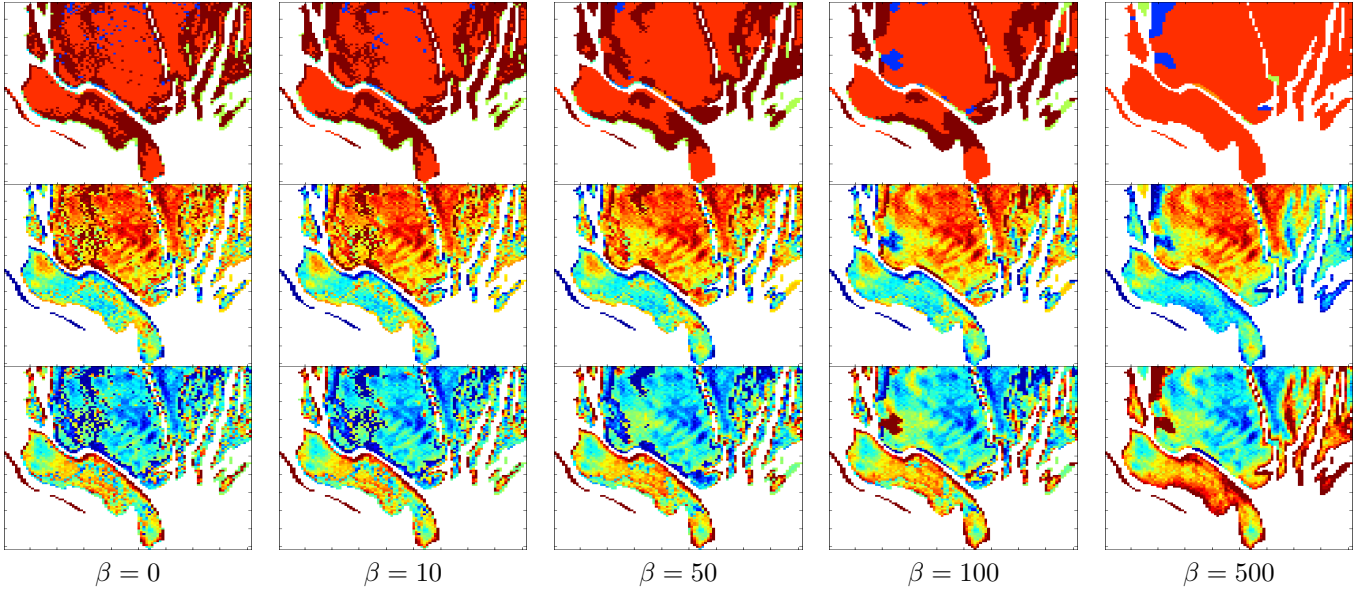
Fig. 3. Qualitative results obtained with MRF-hGLLiM-2 for orbit 41. Top row: Each pixel n is colored according to the class k maximizing p(Z_n = k | Y_n = y_n; \phi) (each class index is assigned an arbitrary color). Middle row: Proportion of CO 2 ice. Bottom row: Proportion of Dust. Concentration color codes are the same as in Fig. 2. To better appreciate the smoothing effect, a zoomed region is shown.
