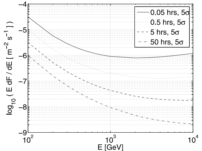
FIG. 4.—Sensitivity of the VERITAS array for exposures of 50, 5, 0.5, and 0.05 hr (i.e., 3 minutes). [See the electronic edition of the Journal for a color version of this figure.]
