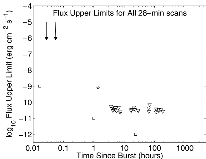
FIG. 3.—Flux upper limits above 400 GeV for all of the GRBs observed (blue triangles). The limits are plotted as a function of time since the GRB prompt emission. The approximate flux level at 400 GeV predicted by Pe’er & Waxman (2004) is indicated by the red solid lines, along with the time interval during which it is predicted to occur. Magenta squares show the emission at 400 GeV predicted by Zhang & Mészáros (2001) at various times after the GRB prompt emission; the prediction of Guetta & Granot (2003a) for VHE emission at 250 GeV 5 \times 10^3 s after the burst from the combination of external Compton and synchrotron self-Compton emission is shown by the black star. [See the electronic edition of the Journal for a color version of this figure.]
