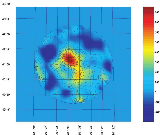
FIG. 3.—Gaussian-smoothed ( \sigma = 7.6' ) declination vs. right ascension map of the excess counts from the TeV J2032+4130 region observed for a total of 65.5 hr between 2003 and 2005. The contours are in steps of 0.5\sigma of the signal significance.
