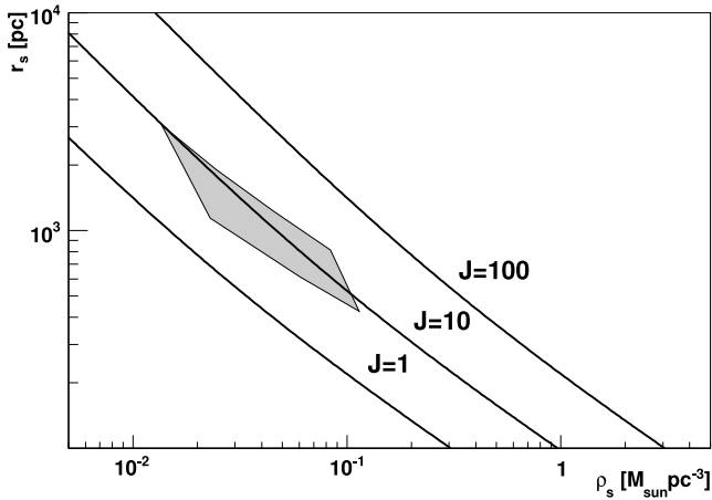
FIG. 5.—Constraints from stellar kinematics data on the parameters r_s and \rho_s of the Ursa Minor DM halo under the assumption of an NFW profile. The gray contour indicates the best-fit mass models of Strigari et al. (2007). Thick solid lines indicate contours of constant J .
