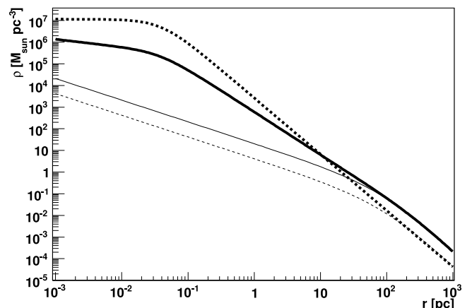
FIG. 7.—M15 DM density profile before ( thin solid line ) and after ( thick solid line ) adiabatic compression modeled as described in the text. Thin and thick dashed lines show the same comparison for the baryonic density profile.
