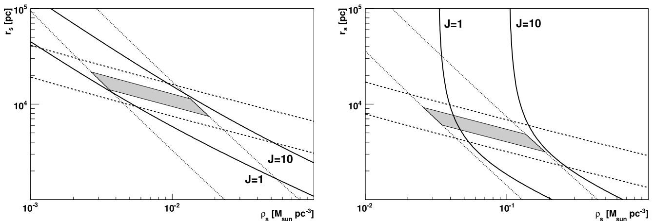
FIG. 9.— Constraints derived using eqs. (9) and (5) for M32 on the parameters r_s and \rho_s of its DM halo under the assumption of an NFW (left) and Burkert (right) profile. Dashed lines show contours of constant virial mass for 10^{11} M_\odot (lower lines) and 10^{12} M_\odot (upper lines). Dotted lines denote the \pm 1 standard deviation bounds on the median halo concentration–to–virial mass relation, eq. (5). Thick solid lines indicate contours of constant J .
