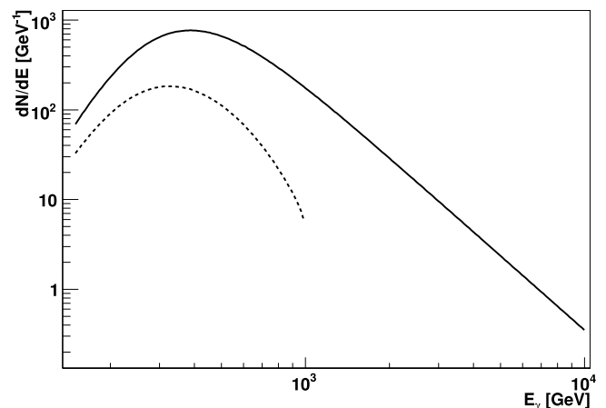
FIG. 3.— Comparison of the differential detection rate of the Crab Nebula (solid line) and a DM halo with \langle\sigma v\rangle = 3 \times 10^{-26} , m_\chi = 1 \text{ TeV} , and J = 10^6 (dashed line). The Supercuts selection criteria are used.
