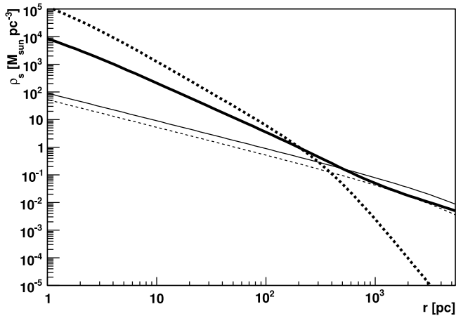
FIG. 10.—Comparison for M32 of the stellar density profile of van der Marel et al. (1998; thick dashed line ) with the modeled DM density profiles before ( thin solid line ) and after ( thick solid line ) adiabatic compression. The thin dashed line shows the assumed initial baryonic density profile.
