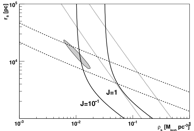
FIG. 11.—Constraints from CO rotation curve data for M33 on the parameters r_s and \rho_s of its DM halo under the assumption of an NFW ( left ) and Burkert ( right ) profile. The gray-shaded region indicates the three standard deviation constraints reported by Corbelli (2003). Dashed lines show contours of constant virial mass for 10^{11} M_{\odot} ( lower lines ) and 10^{12} M_{\odot} ( upper lines ). Dotted lines denote the \pm 1 standard deviation bounds on the median halo concentration-to-virial mass relation, eq. (5). Thick solid lines indicate contours of constant J .
