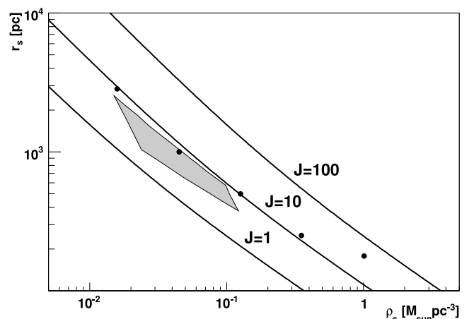
FIG. 4.—Constraints from stellar kinematics data on the parameters r_s and \rho_s of the Draco DM halo under the assumption of an NFW profile. The gray contour and filled circles indicate the best-fit mass models of Strigari et al. (2007) and Mashchenko et al. (2006), respectively. The parameters r_s and \rho_s are defined for the NFW and Burkert halo profiles in eqs. (4) and (6).
