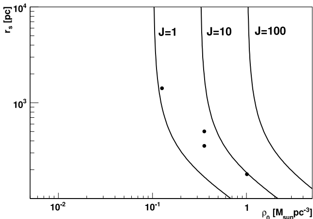
FIG. 6.—Constraints from stellar kinematics data on the parameters r_s and \rho_s of the Draco DM halo under the assumption of a Burkert profile. The filled circles indicate the best-fit mass models of Mashchenko et al. (2006). Thick solid lines indicate contours of constant J .
