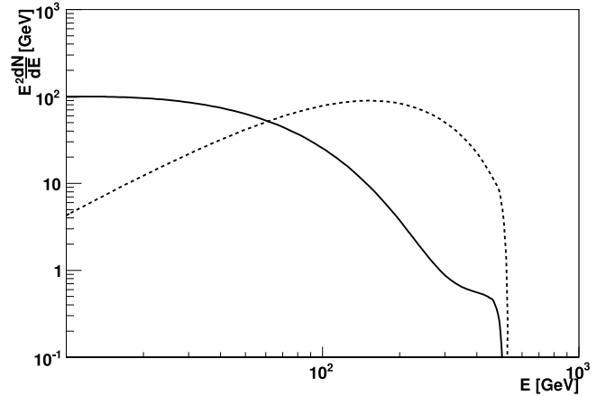
FIG. 1.— Spectral energy density per annihilation for a neutralino of mass 500 GeV annihilating to b\bar{b} (solid line) and \tau^+\tau^- (dashed line). These spectra were generated using the PYTHIA Monte Carlo package (Sjöstrand et al. 2001).
