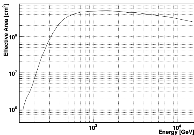
FIG. 2.— Effective area of the Whipple 10 m telescope as a function of energy after selection of gamma-ray–like events with the Supercuts criteria. The effective area below 150 GeV was assumed to be 0 in all computations.
