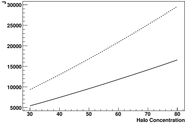
FIG. 8.— Plot of J for the NFW+AC model of M15 as a function of the concentration parameter of the initial DM halo. The solid and dashed lines show the scaling for a DM halo of total virial mass 5 \times 10^6 and 5 \times 10^7 M_\odot , respectively.
