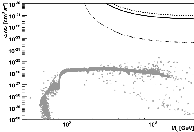
FIG. 12.— Upper limits on \langle\sigma v\rangle as a function of m_\chi calculated using eq. (10) with a composite neutralino spectrum and the J values obtained for the Draco (solid line) and Ursa Minor (dashed line) NFW models and the M15 NFW+AC model (dotted line). Shown as open circles are MSSM models that fall within \pm 3 standard deviations of the relic density measured in the 3 yr WMAP data set (Spergel et al. 2007). [See the electronic edition of the Journal for a color version of this figure.]
