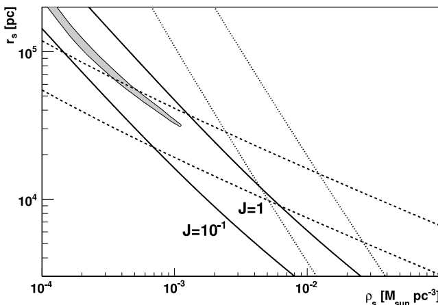
FIG. 11.—Constraints from CO rotation curve data for M33 on the parameters r_s and \rho_s of its DM halo under the assumption of an NFW ( left ) and Burkert ( right ) profile. The gray-shaded region indicates the three standard deviation constraints reported by Corbelli (2003). Dashed lines show contours of constant virial mass for 10^{11} M_{\odot} ( lower lines ) and 10^{12} M_{\odot} ( upper lines ). Dotted lines denote the \pm 1 standard deviation bounds on the median halo concentration-to-virial mass relation, eq. (5). Thick solid lines indicate contours of constant J .
