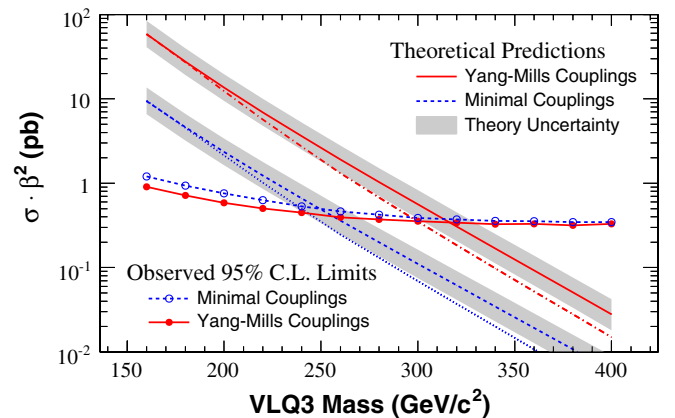
FIG. 2 (color online). The 95% C.L. upper limits on \sigma(p\bar{p} \rightarrow VLQ3VLQ3) \cdot \beta^2 versus mass (lines with symbols), where \beta \equiv \mathcal{B}(VLQ3 \rightarrow b\tau) . The theoretical expectations are shown for the Yang-Mills (solid line) and minimal (dashed line) couplings scenarios for the case \beta = 1 , with bands for uncertainties due to the choices of PDFs and Q^2 . The dot-dashed and dotted curves show the threshold effect when the VLQ3 \rightarrow \nu_\tau t channel is open.
