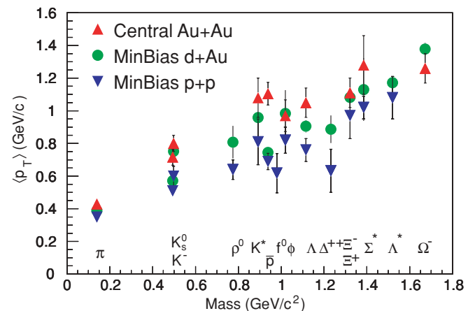
FIG. 28. (Color online) \langle p_T \rangle of various particles for different systems, minimum bias p+p and d+Au , and central Au+Au collisions. The errors shown are the quadratic sum of the statistical and systematic uncertainties.
