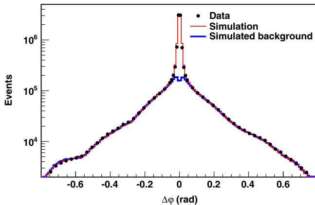
FIG. 2 (color online). Distribution of the azimuthal separation ( \Delta\varphi ) of all candidate tracklets in data, simulation, and the background contribution that is estimated from the simulation.
