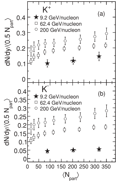
FIG. 11. dN/dy of (a) K^+ and (b) K^- , normalized by \langle N_{\text{part}} \rangle/2 for Au + Au collisions at \sqrt{s_{NN}} = 9.2 GeV, plotted as a function of \langle N_{\text{part}} \rangle . The lower energy results are compared with corresponding results for Au + Au collisions at \sqrt{s_{NN}} = 62.4 and 200 GeV [4,23,37]. The errors shown are the quadrature sum of statistical and systematic uncertainties. The systematic errors on K^+ and K^- yields for \sqrt{s_{NN}} = 9.2 GeV data are similar, about 18% for all the collision centralities studied.
