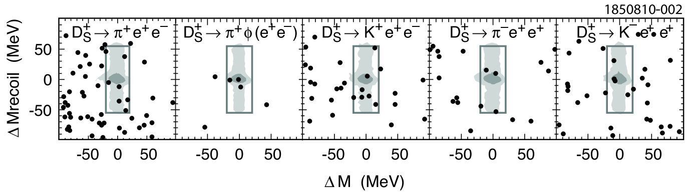
FIG. 2 (color online). Scatterplots of \Delta M_{\text{recoil}} vs \Delta M . The two contours for each mode enclose regions determined with signal MC simulation to contain 40% and 85% of signal events, respectively. The signal region, defined by (\Delta M, \Delta M_{\text{recoil}}) = (\pm 20 \text{ MeV}, \pm 55 \text{ MeV}) , is shown as a box.
