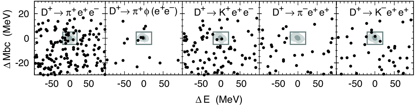
FIG. 1 (color online). Scatterplots of \Delta M_{bc} vs \Delta E . The two contours for each mode enclose regions determined with signal MC simulation to contain 50% and 85% of signal events, respectively. The signal region, defined by (\Delta E, \Delta M_{bc}) = (\pm 20 \text{ MeV}, \pm 5 \text{ MeV}) , is shown as a box.
