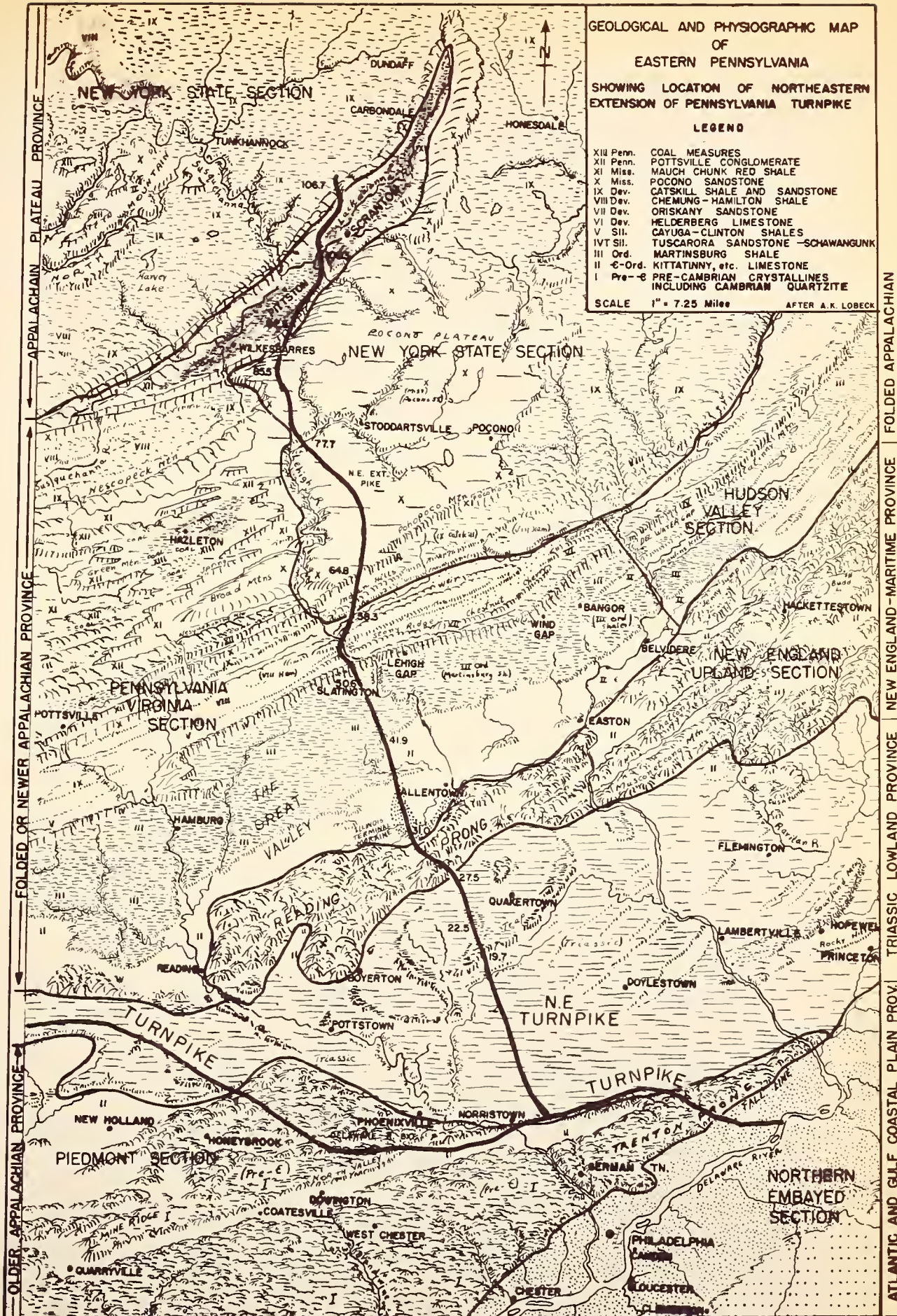
FIG. 3 GEOLGIC. AND PHYSIOGRAPHIC MAP OF NORTHEASTERN PENNSYLVANIA
