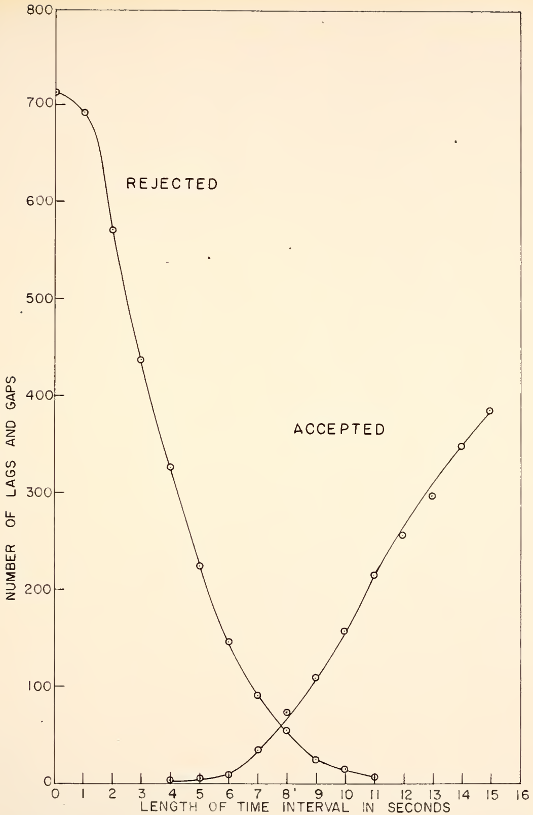
FIGURE 3 DISTRIBUTION OF ACCEPTED AND REJECTED LAGS AND GAPS AT INTERSECTION (A AND B). LEFT TURNS.
