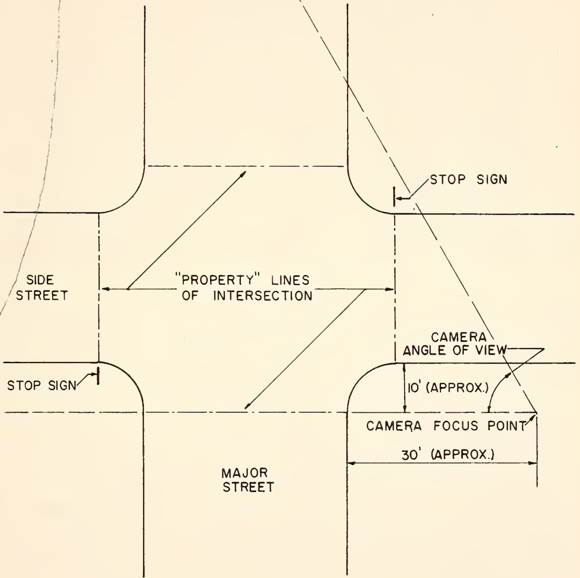
FIGURE 1 TYPICAL FIELD SETUP
