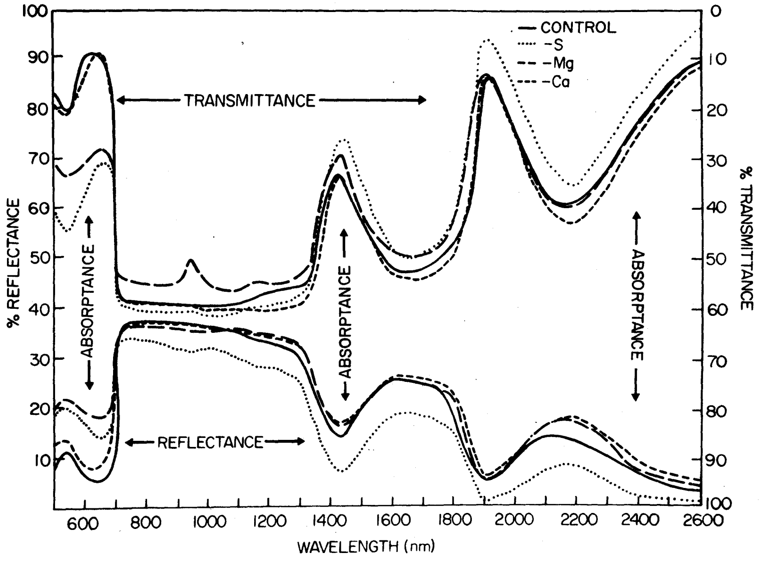
Figure 3. The relationship between the absolute spectral reflectance, transmittance, and absorptance for control, Ca-, Mg-, and S-deficient maize leaves between 500-2600 nm.
