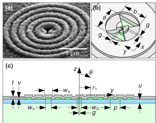
FIG. 1. (Color online) Structure geometry. (a) SEM image showing aluminum surface and bowtie aperture and [(b) and (c)] schematic of aperture and grating geometry.
