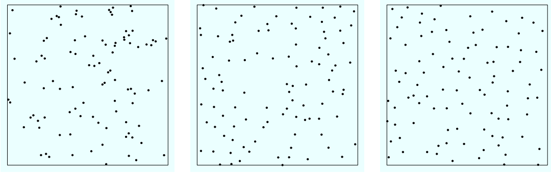
Figure 1: From left to right, letting the intensity \rho = 100 , realizations on [0, 1]^2 of a stationary Poisson process, a DPP with a Gaussian kernel and the maximal possible choice for the range parameter \alpha ( \alpha = 0.056 ), a DPP with kernel (2.2).
