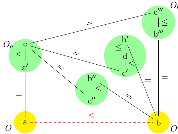
Figure 3.1: 2-context traversal. Of the three paths found between a and b , two return the \leq relation and the third one returns all the possible relations ( \Gamma ).
