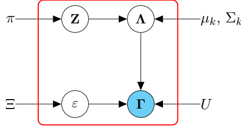
FIG 3.1. Graphical representation for the model \text{DFM}_{[\Sigma_k \beta]} .
