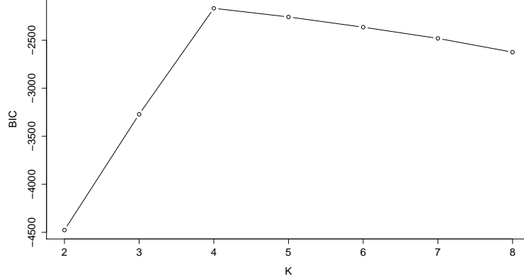
FIG 4.2. Selection of the number of clusters using BIC on the simulated data (actual value of K is 4).
