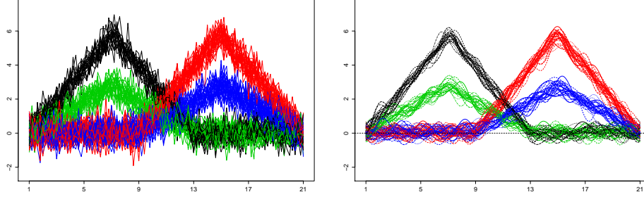
FIG 4.1. Raw and smoothed simulated curves.
