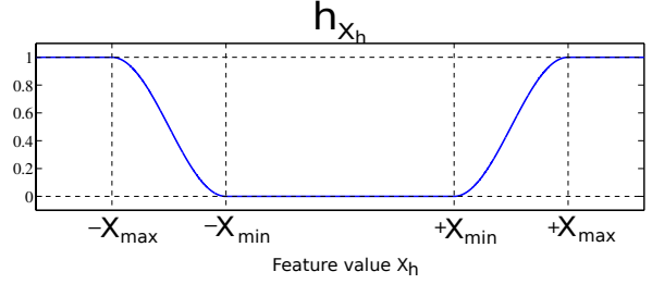
Fig. 7. The evolution of h_{X_h} with respect to the feature X_h
