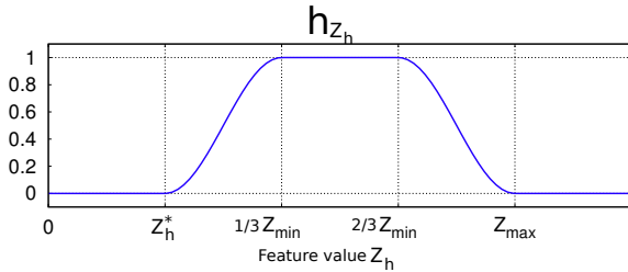
Fig. 6. The evolution of h_{Z_h} with respect to the feature Z_h
