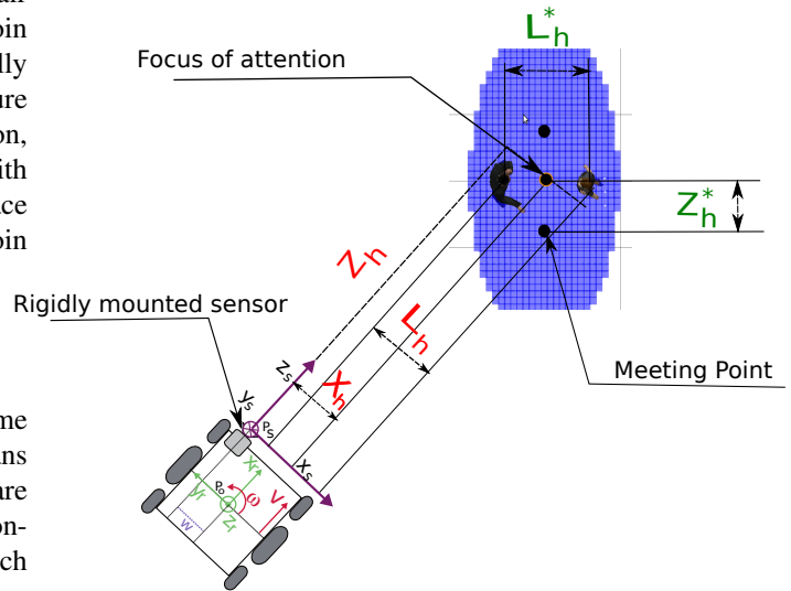
Fig. 4. A unicycle-type robot with respect to an interacting group. Robot and sensor frames along with the geometric representation of the task features are shown.
