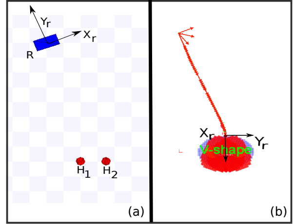
Fig. 11. Scenario 1: The initial position of the robot with respect to the humans H_1 and H_2 (a) and the trajectory taken by the robot in order to reach the meeting point (b)
