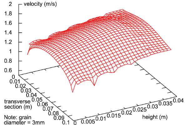
Figure 1: velocity profile
