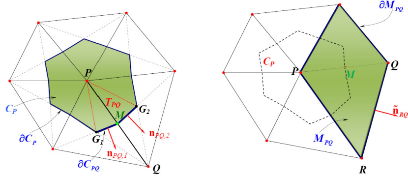
Figure 1: Median-dual computational cell (left) and computational cell for the gradient of the divergence (right)
