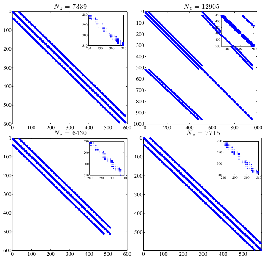
Figure 3: Sparsity patterns for the different mesh types for N_x = 15
