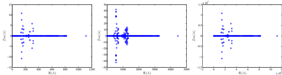
Figure 5: Eigenvalues of three matrices using the Orthogonal I type of grid. \frac{h}{h_N} = \frac{1}{0.0456} (left), \frac{1}{0.0232} (middle), \frac{100}{0.0456} (right)
