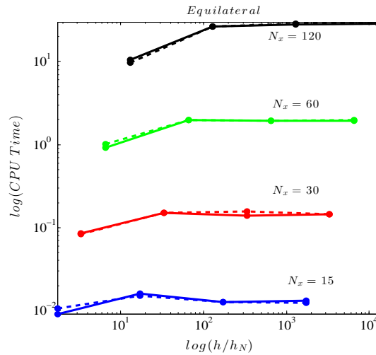
Figure 8: CPU time versus h/h_N for GMRES (solid line) and BiCGStab (dashed line) applying the ILUT preconditioner with \tau = 10^{-5} .
