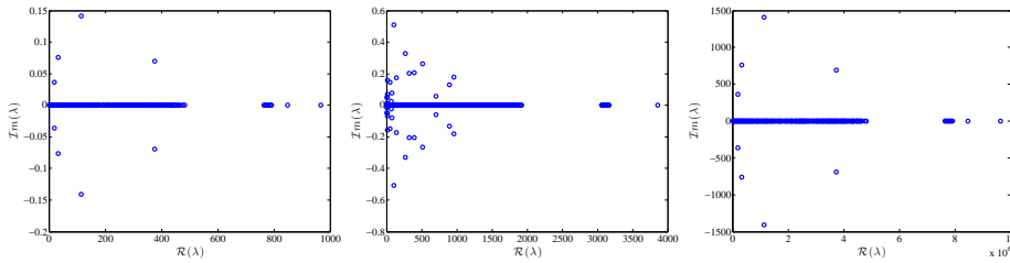
Figure 4: Eigenvalues of three matrices using the equilateral type of grid. \frac{h}{h_N} = \frac{1}{0.058} (left), \frac{1}{0.031} (middle), \frac{100}{0.058} (right)
