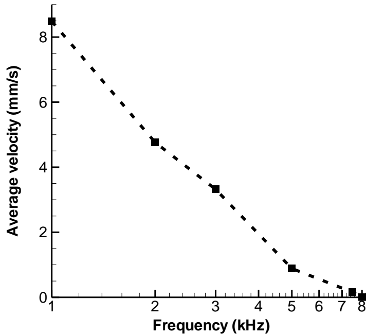
Figure 10. Average velocity of a 2 mm-diameter ethylene glycol droplet under an AC voltage of magnitude 50 V versus AC frequency.
