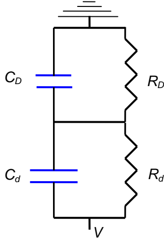
Figure 3. RC network used to estimate the actuation force on a generic liquid droplet.
