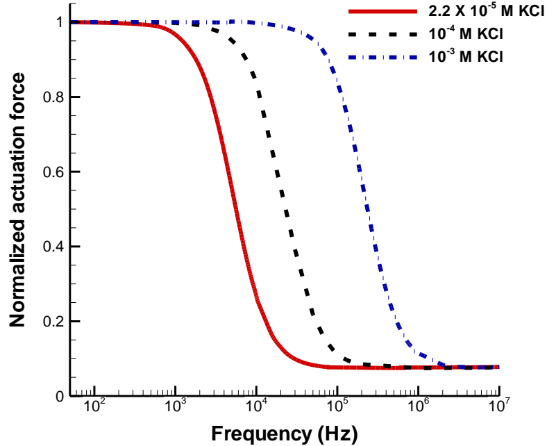
Figure 4. Normalized frequency-dependent actuation force for KCl solutions.
