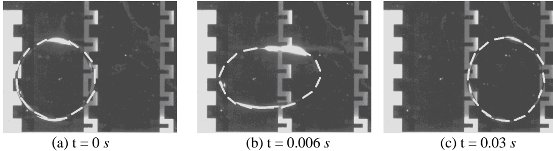
Figure 6. Transition of a 2 mm-diameter 10^{-3} M KCl droplet under an AC voltage of magnitude 50 V and frequency 50 Hz; the outline of the droplet has been highlighted with a dashed line for easier recognition.
