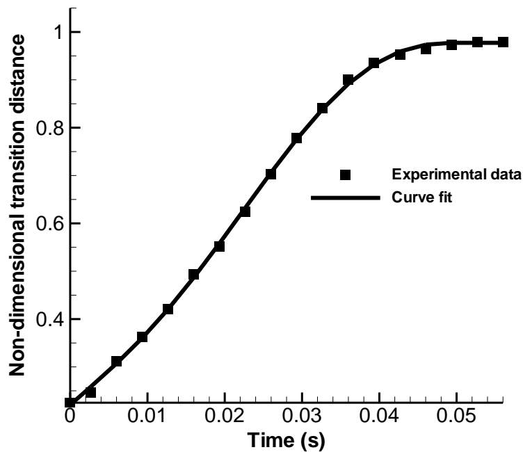
Figure 7. Transition position variation of a 2 mm-diameter 10^{-3} M KCl droplet under an AC voltage of magnitude 50 V and frequency 5 kHz.
