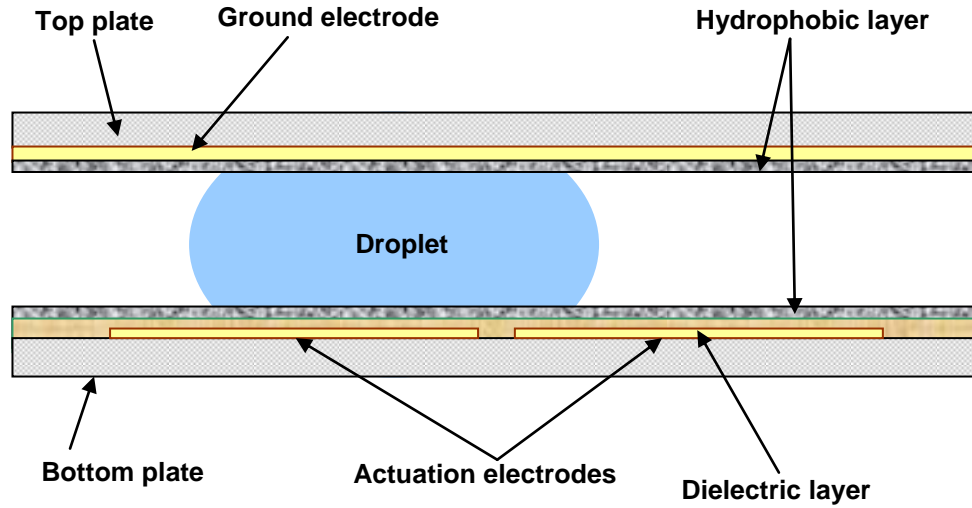
Figure 1. Representative device for electrical actuation of droplets [10].
