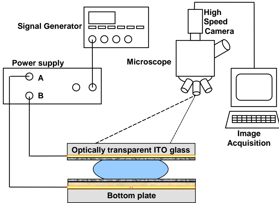
Figure 5. Schematic of the experimental setup used for measurement of droplet velocities.
