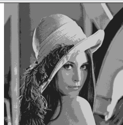
K-means quantization
