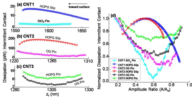
FIG. 6. (Color online) [(a)–(c)] Dissipation per oscillation cycle for the three CNT AFM probes in Fig. 2 on different samples. Only data in the intermittent contact regime are shown. In general, dissipation is larger on HOPG than either SiO 2 or OG for a given tip with similar parameters. Slipping dissipation is not only significantly larger but displays a concave down dependence as opposed to the constant dissipation during pinning. (d) When the dissipation curves are normalized to distinguish between the different dissipative mechanisms (Ref. 61), the presence of a different dissipation mechanism due to CNT slipping is clear from the concave up, amplitude-dependent shape for CNT1 and CNT2 on HOPG contrasted with the nearly flat dissipation when CNTs are pinning.
