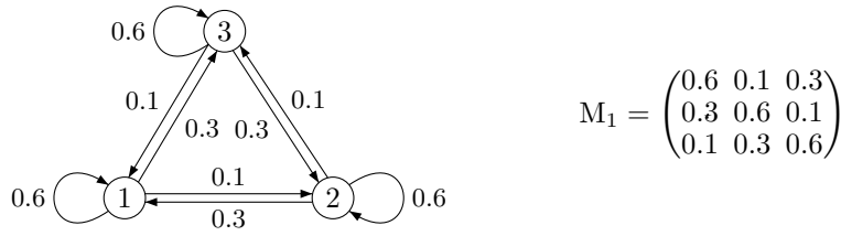
Fig. 5. An irreducible and aperiodic Markov chain with its transition matrix M_1
