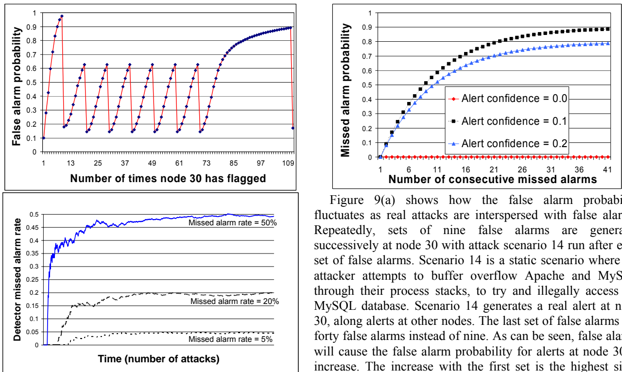
Figure 9. Behavior of false and missed alarm computation algorithms
