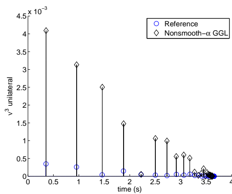
Figure 11: Bouncing pendulum: unilateral multiplier \nu^3 .
