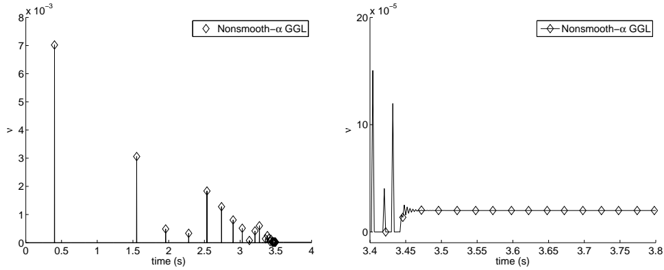
Figure 7: Bouncing ball: Lagrange multiplier \nu and zoom.
