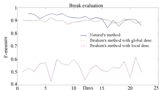
Fig. 2. Results in terms of break F-measure.
