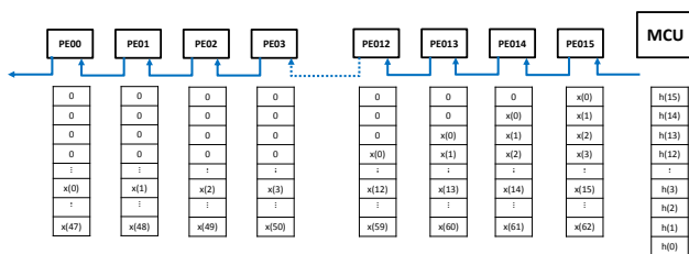
Figure 11: FIR filter implementation in 1D-configuration
