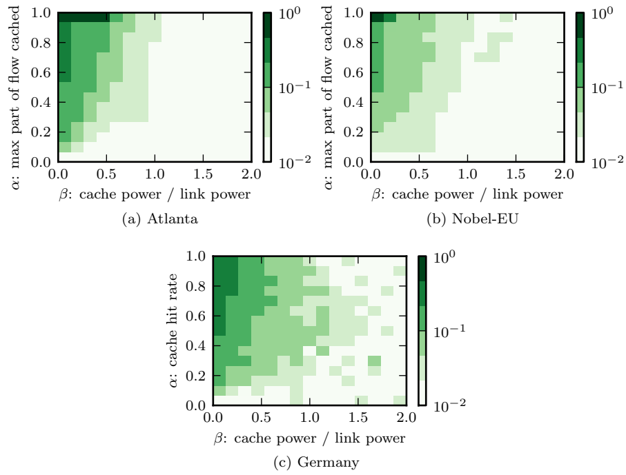
Figure 5 – Part of power consumption saved by introducing caches with various parameters. Baseline is network power consumption without cache.
