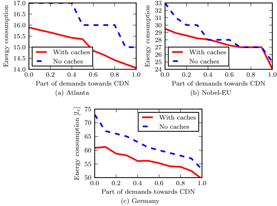
Figure 7 – Impact of caches and CDN cooperation on energy consumption
