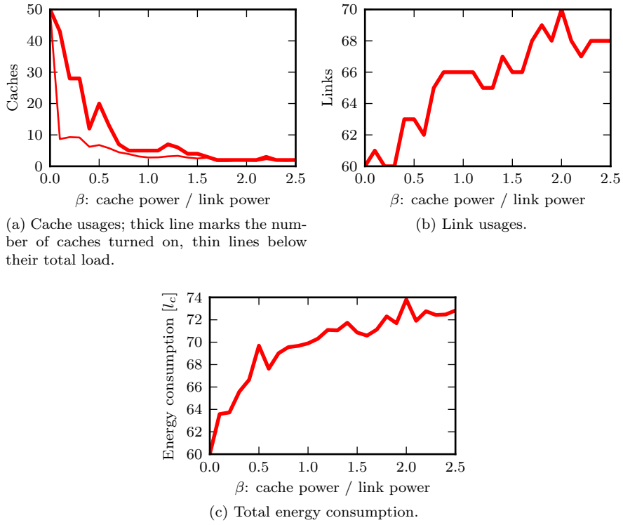
Figure 4 – Results as a function of parameter \beta (cache power / link power) for Germany50 .
