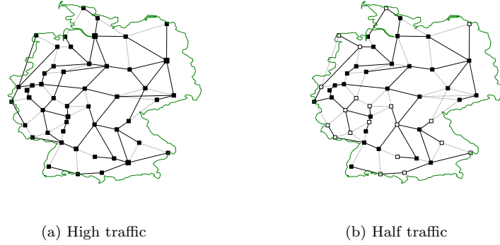
Figure 10 – Breakdown of devices used for two levels of traffic (Right has half the traffic of left).
