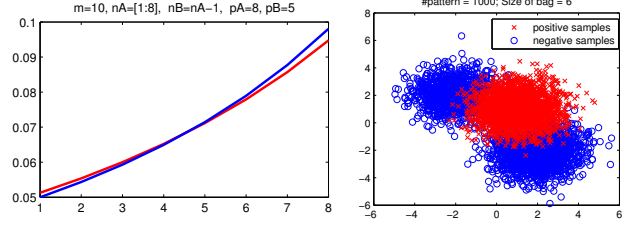
Figure 1: Plots of Eq. (31) Figure 2: The data (red) and Eq. 32 (blue) as a for the synthetic problem of n_A . As these two lem. The negative samples are drawn from a mixture of Gaussians. plots cross, neither function bounds the other.
