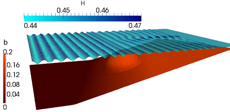
Figure 15: Test 5 - Periodic waves propagation over an elliptic shoal: topography and view of the free surface.
