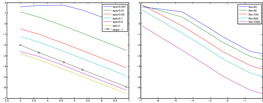
Figure 10: Plot of the \ell^\infty error for the new method with corrected initial condition and numerical approximation for S . Left: error (log-log scale) as a function of N_{ts} ( N_{ts} = 20, 40, 100, 200, 1000 ) for different values of \varepsilon ( \varepsilon = 1, \dots, 10^{-3} ). Right: error (log-log scale) as a function of \varepsilon for different N_{ts} .
