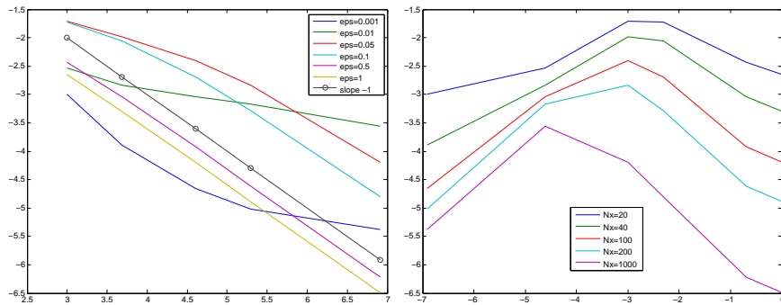
Figure 12: Plot of the \ell^\infty error for the new method without corrected initial condition and an exact computation for S . Left: error (log-log scale) as a function of N_{ts} ( N_{ts} = 20, 40, 100, 200, 1000 ) for different values of \epsilon ( \epsilon = 1, \dots, 10^{-3} ). Right: error (log-log scale) as a function of \epsilon for different N_{ts} .
