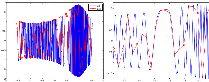
Figure 7: Comparison between a reference solution and the solution of the new method ( with initial correction and exact computation for S ), for \varepsilon = 5 \cdot 10^{-3} , t_f = 1 . Left: space dependence of the real part of the unknown. The right part is a zoom of the left part.
