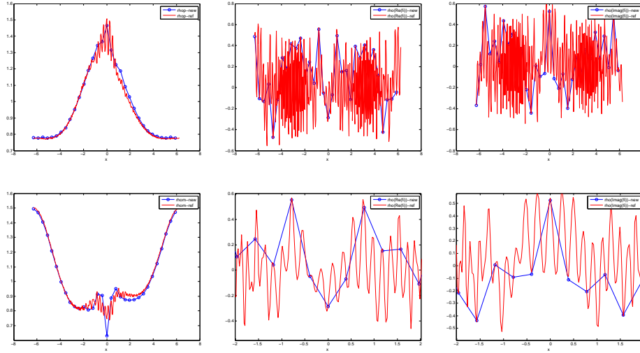
Figure 17: \varepsilon = 1/32 . First line: space dependence of the densities \rho^+ , \text{Re}(\rho^i) and \text{Im}(\rho^i) . Second line: space dependence of \rho^- , \text{Re}(\rho^i) (zoom) and \text{Im}(\rho^i) (zoom).
