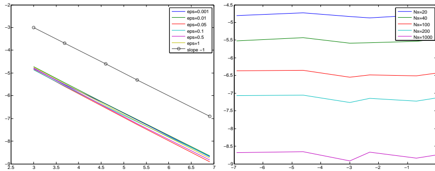
Figure 3: Plot of the \ell^\infty error for the new method with corrected initial condition and an improved numerical approximation for S (pseudo-spectral in space and 4th order Runge-Kutta). Left: error (log-log scale) as a function of N_{ts} ( N_{ts} = 20, 40, 100, 200, 1000 ) for different values of \epsilon ( \epsilon = 1, \dots, 10^{-3} ). Right: error (log-log scale) as a function of \epsilon for different N_{ts} .
