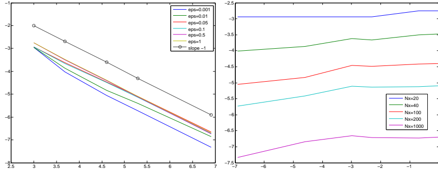
Figure 11: Plot of the \ell^\infty error for the new method with corrected initial condition and an improved numerical approximation for S (pseudo-spectral in space and 4th order Runge-Kutta). Left: error (log-log scale) as a function of N_{ts} ( N_{ts} = 20, 40, 100, 200, 1000 ) for different values of \epsilon ( \epsilon = 1, \dots, 10^{-3} ). Right: error (log-log scale) as a function of \epsilon for different N_{ts} .
