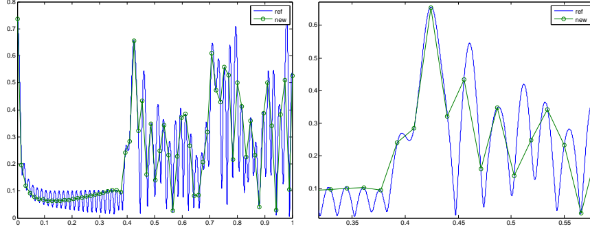
Figure 8: Time history of \mathcal{R} . Comparison between a reference solution and the solution of the new method ( with initial correction and exact computation for S ), for \varepsilon = 5 \cdot 10^{-3} , t_f = 1 . The right part is a zoom of the left part.
