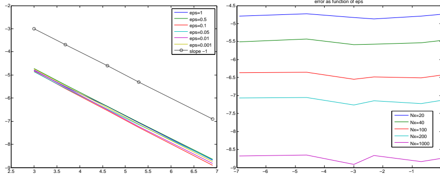
Figure 1: Plot of the \ell^\infty error for the new method with corrected initial condition and exact computation for S . Left: error (log-log scale) as a function of N_{ts} ( N_{ts} = 20, 40, 100, 200, 1000 ) for different values of \epsilon ( \epsilon = 1, \dots, 10^{-3} ). Right: error (log-log scale) as a function of \epsilon for different N_{ts} .
