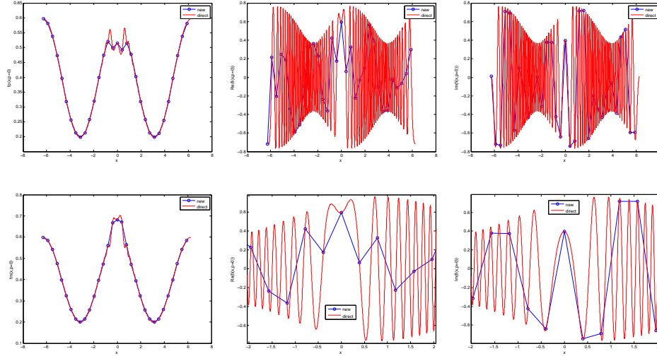
Figure 18: \varepsilon = 1/256 . First line: space dependence of f^+ , \text{Re}(f^i) and \text{Im}(f^i) at p = 0 . Second line: space dependence of f^- , \text{Re}(f^i) (zoom) and \text{Im}(f^i) (zoom) at p = 0 .
