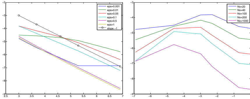
Figure 4: Plot of the \ell^\infty error for the new method without corrected initial condition and exact computation for S . Left: error (log-log scale) as a function of N_{ts} ( N_{ts} = 20, 40, 100, 200, 1000 ) for different values of \varepsilon ( \varepsilon = 1, \dots, 10^{-3} ). Right: error (log-log scale) as a function of \varepsilon for different N_{ts} .
