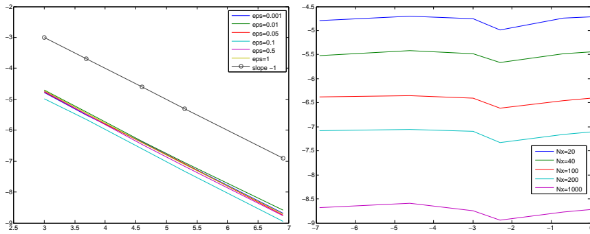
Figure 5: Plot of the \ell^\infty error for the new method with corrected initial condition and exact computation for S , in the case where a vanishes ( a(x) = 1 + \cos(2x) ) at isolated points. Left: error (log-log scale) as a function of N_{ts} ( N_{ts} = 20, 40, 100, 200, 1000 ) for different values of \varepsilon ( \varepsilon = 1, \dots, 10^{-3} ). Right: error (log-log scale) as a function of \varepsilon for different N_{ts} .
