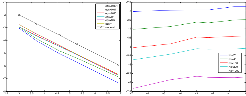
Figure 9: Plot of the \ell^\infty error for the new method with corrected initial condition and exact computation for S . Left: error (log-log scale) as a function of N_{ts} ( N_{ts} = 20, 40, 100, 200, 1000 ) for different values of \varepsilon ( \varepsilon = 1, \dots, 10^{-3} ). Right: error (log-log scale) as a function of \varepsilon for different N_{ts} .
