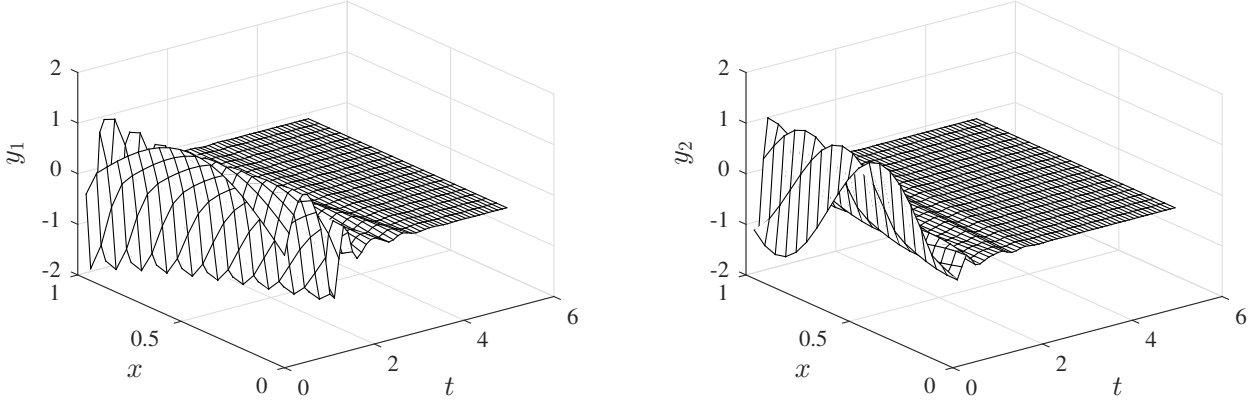
FIGURE 4. Evolution of the first component y_1 (left) and of the second component y_2 (right) of system (1)–(3) with \Lambda and F given, respectively, by (76) and (77), initial condition given by (79), and under the boundary control (78).
