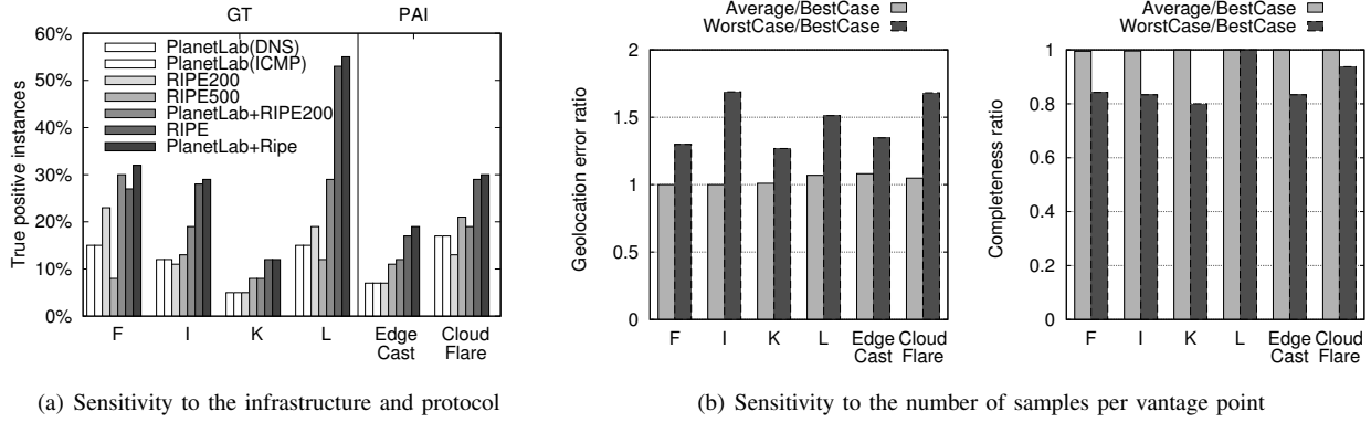
Fig. 7. Sensitivity of iGreedy to the measurement infrastructure and campaigns: (a) impact of vantage point combinations and network protocols; (b) best, average and worst-case results with P = 100 measurement per vantage point.
