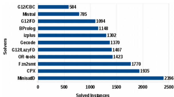
Figure 1: Total number of solved instances for each solver of the portfolio.
