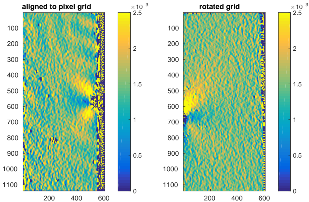
Figure 8: Real-case study. Retrieved strain map \varepsilon_{xx} from the aligned-to-pixel grid (on the left) and from the rotated grid (on the right). The large parasitic fringes that can be seen on the left are not present on the right. These fringes are caused by aliasing. Note the effect of the noise, inherent to any digital acquisition device.
