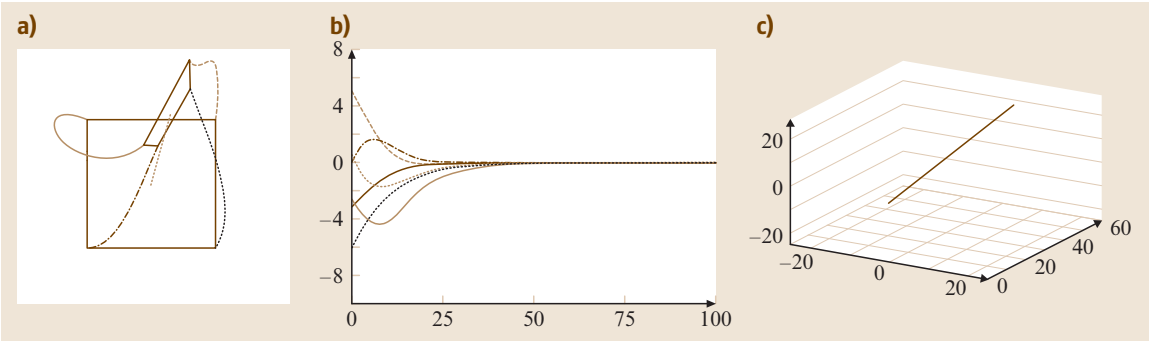
Figure 34.13: 2.5D VS system behavior using s = ({}^c t_c, \mathbf{x}_g, \theta_{u_z})
