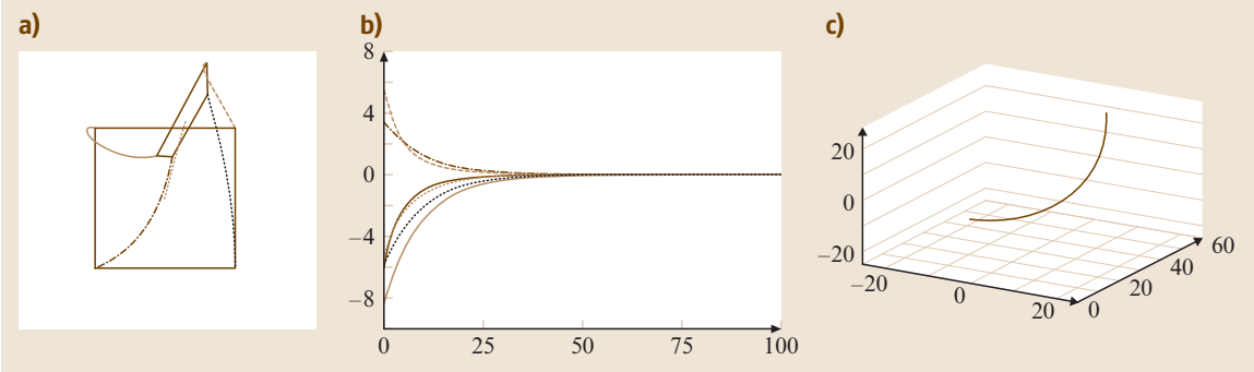
Figure 34.12: 2.5D VS system behavior using s = (\mathbf{x}_g, \log(Z_g), \theta_u)
