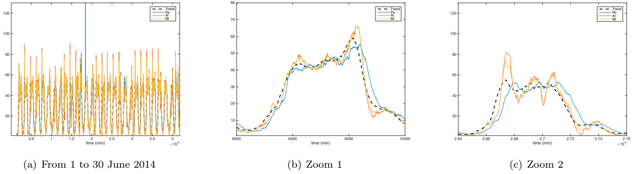
Fig. 4. 15 minutes forecasts
